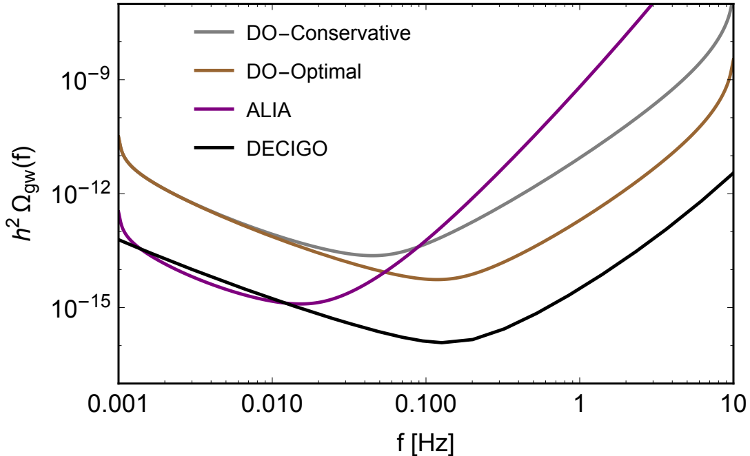
Figure 5. Ability to detect a stochastic gravitational-wave background, characterised by the power-law sensitivity h^2 \Omega_{\text{GW}}(f) [401–403]. Sensitivities are calculated assuming a 4 yr mission with a 70% efficiency, and a required signal-to-noise ratio threshold of 10.
