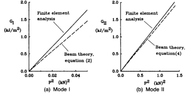
Fig. 13 G_I and G_{II} components from beam-theory and finite-element analysis.
