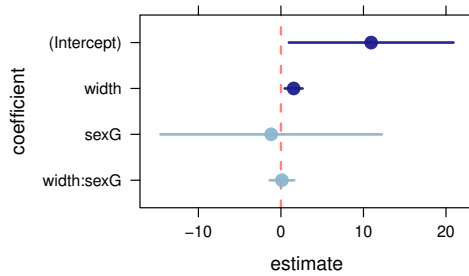
95% confidence intervals
