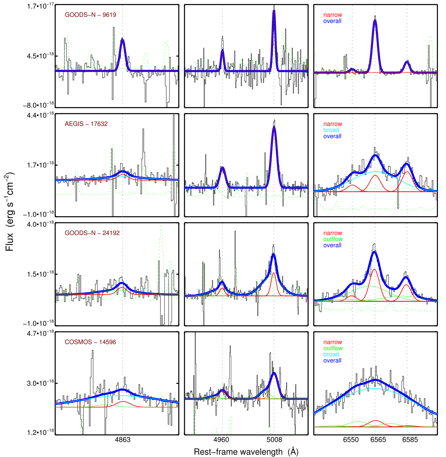
Figure 3. Examples of MOSDEF spectra and the multiple-component fitting procedure for four AGNs in our sample (the IDs are from v4.1 of the 3D- HST catalogs). The overall fit is shown in blue, while the individual Gaussian components are shown in different colors: red for the narrow component, green for an outflow, and cyan for a broad component. The error spectra are shown with dotted green lines, while vertical dotted gray lines show the rest frame wavelength of the emission lines we fit. The top row shows an AGN where only a narrow Gaussian component is required to fit all of the lines. The second row shows an AGN that requires an additional broad component to fit H\beta and H\alpha . The third row shows an AGN with a clear outflow component, detected in the [O\ III] and H\alpha lines. The fourth row shows an AGN that requires both an outflow component (seen in [O\ III]\ \lambda 5008 ) and a broad component. Sources that have a broad H\alpha and/or H\beta component with the S/N > 3 are excluded from our analysis in Section 3, as we cannot reliably probe their host galaxy properties.
