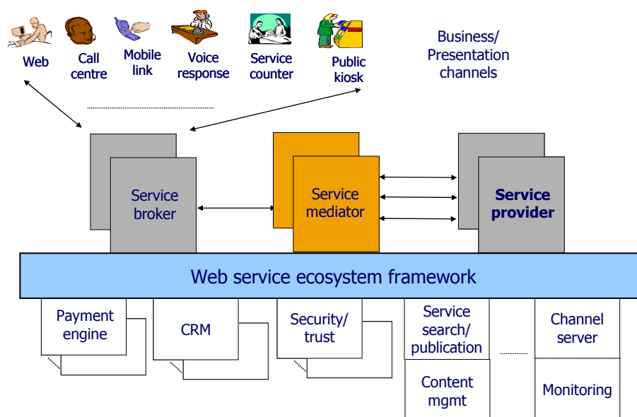
Figure 1. Service supply and distribution supported in a web service ecosystem framework
