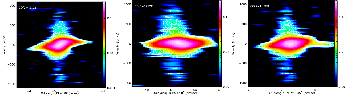
Fig. 6. Position-velocity plots with east-west ( left panel , left to right), south-north ( middle panel , left to right) and PA -45^\circ , south-west to north-east ( right panel , left to right) cuts, through the CO(2–1) peak from DS1. Contours levels are 3 to 15\sigma , 1\sigma = 1.3 mJy/20 MHz.
