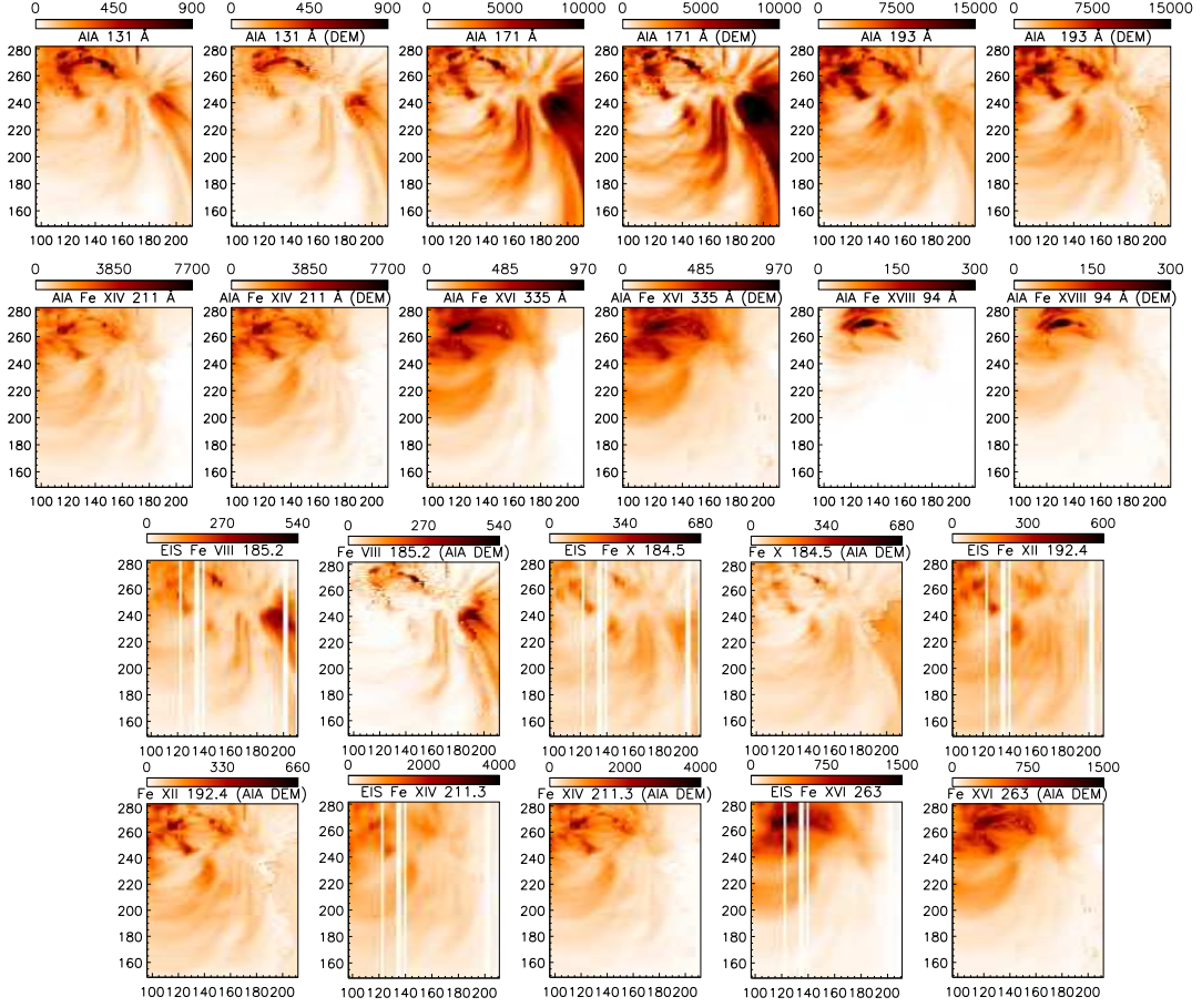
Fig. 4. Top two rows: observed and estimated (from the AIA DEM modelling) AIA images (negative, DN/s) of the on-disk AR observation of 2010 Oct 26, rebinned to the EIS resolution. Lower two rows: monochromatic images (negative, photons \text{cm}^{-2} \text{s}^{-1} \text{arcsec}^{-2} ) in EIS lines, observed and estimated from the AIA DEM modelling.
