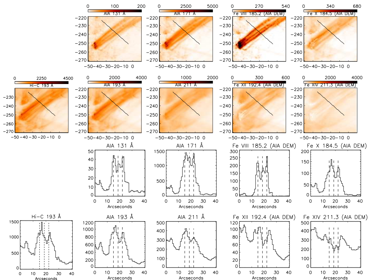
Fig. 15. Above: the region R3, as observed Hi-C, by AIA, and as predicted from the AIA DEM modelling. Below: profiles (averages over 1.8'' in DN/s) along the segment indicated in the images. The position of a few cool loops is noted.
