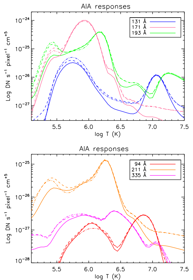
Fig. 1. The SDO AIA response functions calculated with the present atomic data, the present ‘coronal’ abundances and a constant electron density of 2 \times 10^9 \text{ cm}^{-3} (full lines). The dashed lines are the responses calculated with ‘photospheric’ abundances, multiplied by 3.16. The dash dot lines are calculated with CHIANTI v.7.1, and ‘photospheric’ abundances multiplied by 3.16.
