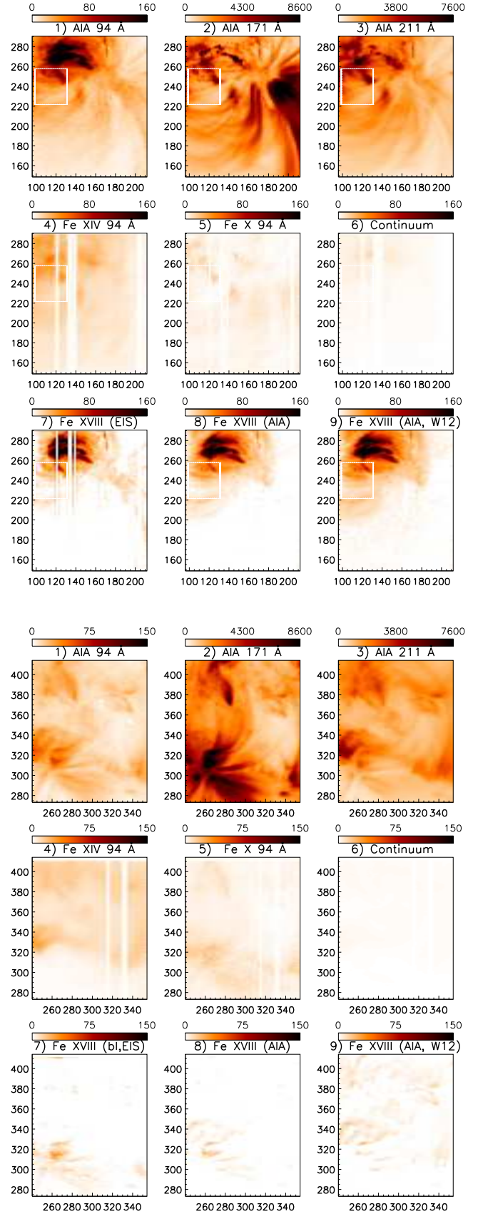
Fig. 7. AIA images (negative, DN/s/pixel) of the on-disk AR observations of 2010 Oct 26 (above) and Nov 23 (below), rebinned onto the EIS resolution. Panels 4,5,6 show the 94 Å predicted count rates in Fe XIV, Fe X, and the continuum. Panels 7 and 8 show the residual count rates in the AIA 94 Å (due to Fe XVIII), estimated from EIS and AIA. Panels 9 show the Fe XVIII estimate of Warren et al. (2012).
