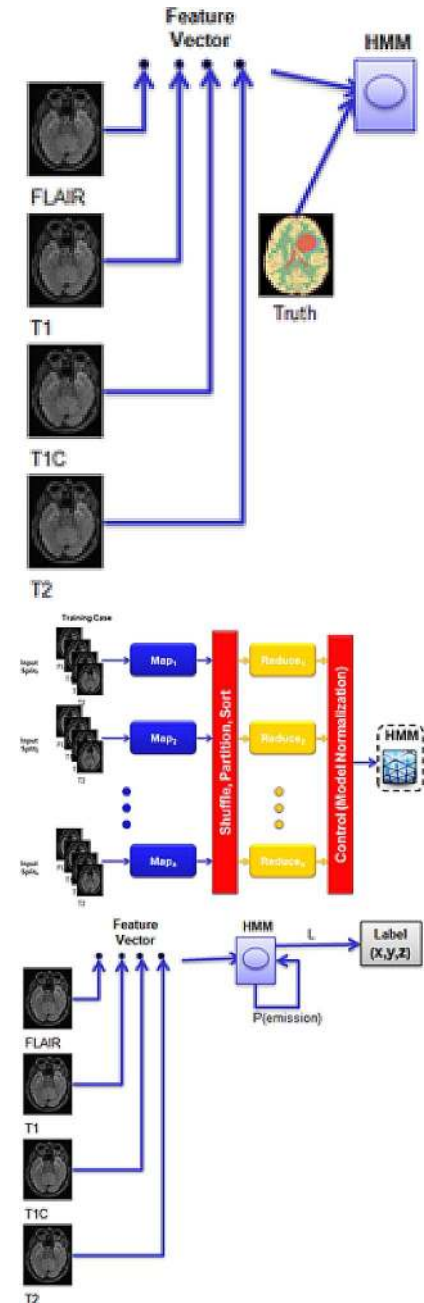
Fig. 12. Left: Training the HMM model. Center: MapReduce model for HMM-based brain tumor segmentation. Right: Applying the HMM model for segmentation.
