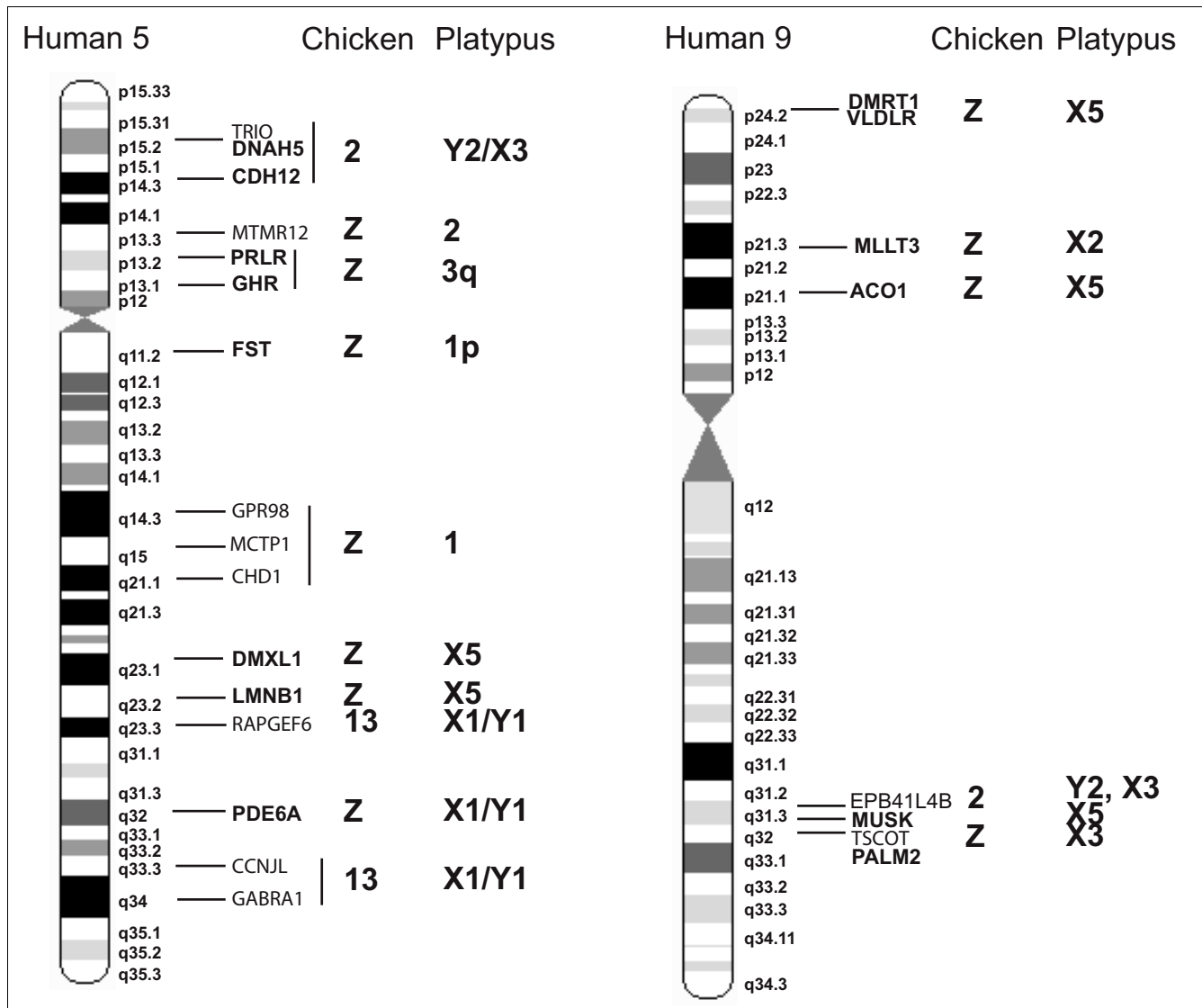
Figure 11 Location of mapped human 5 and human 9 genes in human, chicken and platypus. Gene names in italic are mapped in platypus by PCR, gene names in bold are mapped by both PCR and BAC-clone FISH. EPB41L4B is in contig 29 (Additional data file 1, P15RS).
