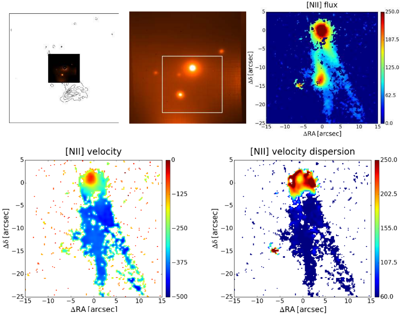
Fig. 8. 3C 318.1, complex radio morphology, no optical spectroscopic classification, FR II/HEG, 1'' = 0.90 kpc. Top left : radio contours overlaid onto the Muse optical continuum image. Top center : Muse optical continuum image. Top right : [N II] emission line image extracted from the white square in the top center panel. Middle : velocity field and velocity dispersion from the [N II] line.
