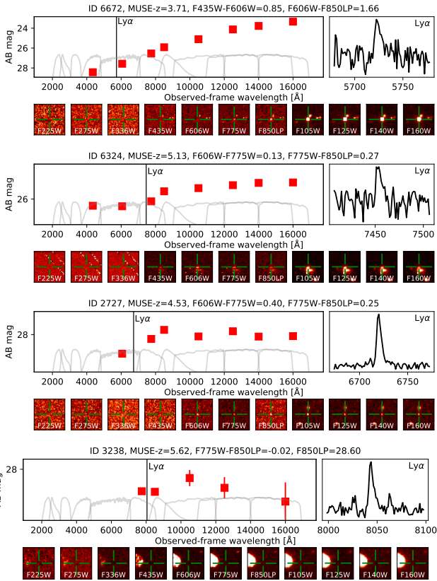
Fig. 26. Examples of the outliers in the F435W (top panel), F606W (two middle panels), and F775W (bottom panel) dropout selections. In each panel, a spectral energy distribution using the HST photometries is shown at the top left, a zoomed-in part of the Ly \alpha detected wavelength region is presented at the top right, and thumbnail HST images of the object are shown at the bottom. The object ID, MUSE spec- z , and the colors of each galaxy can be found at the top of each panel.
