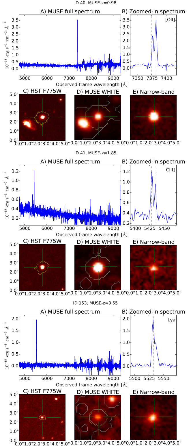
Fig. 5. Full MUSE spectrum and a zoomed-in portion of the [OII], CIII], and \text{Ly}\alpha detected wavelength region at the top of each panel, and the HST F775W, MUSE white-light, and narrowband images of each emission line in the bottom of each panel. The yellow contours in the images are the boundary of the UVUDF catalog segmentation for the object, but those in the MUSE white-light image are convolved with the MUSE beam size. The white boundaries indicate masked objects excluded from local sky residual estimates. The green cross indicates the central position of the extracted object. The ID numbers and measured redshift are indicated at the top of each panel. All of these redshifts are secure ( \text{CONFID} = 2 or 3).
