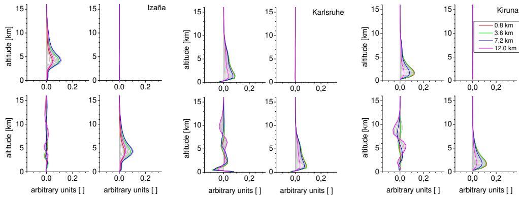
Figure 4. Same as Fig. 2 but for the a posteriori corrected {humidity, δD} proxy state (kernel matrix A'' according to Eq. 7).
