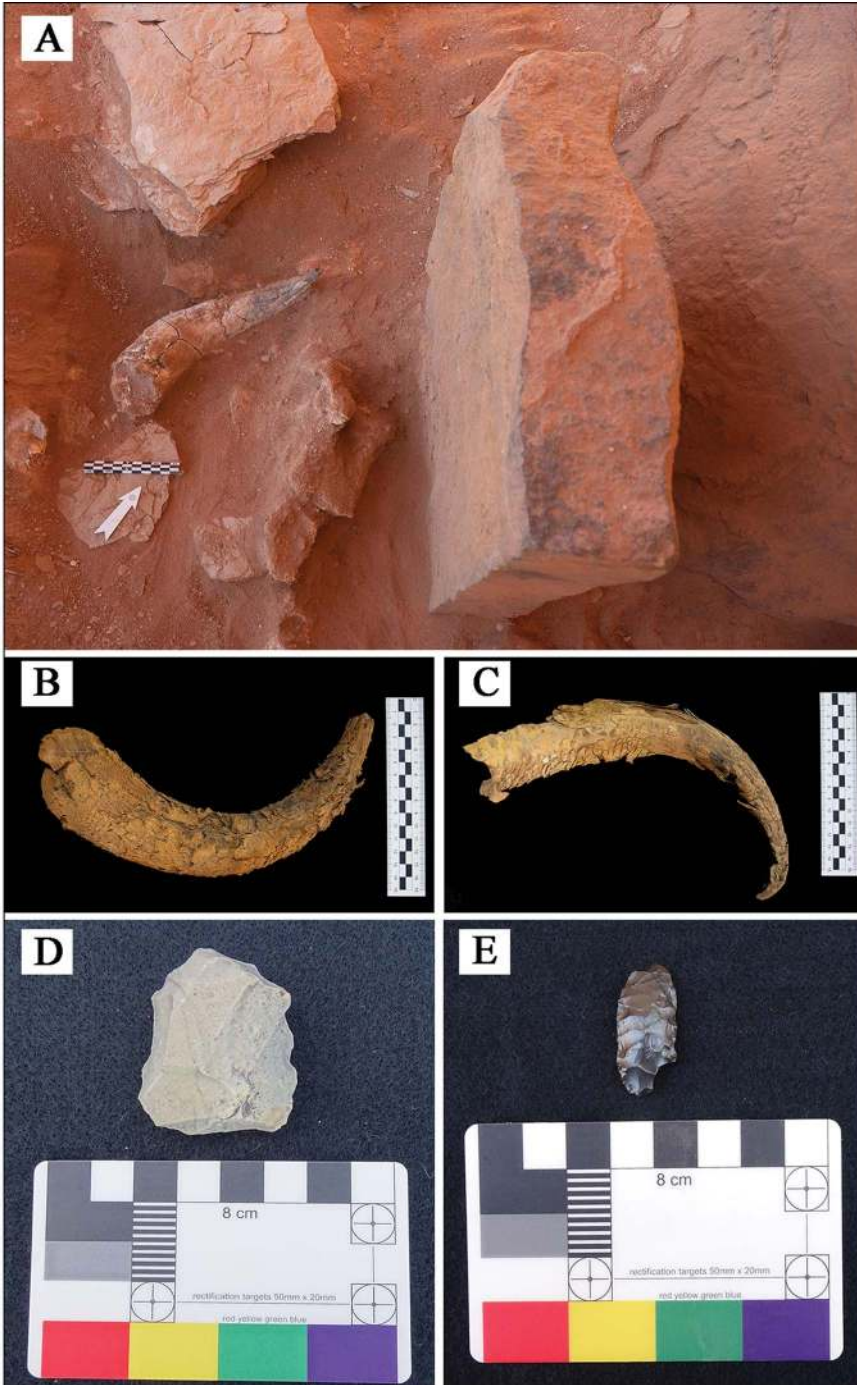
Figure 9. Artefacts recovered during excavation and ground survey: A) cattle horn positioned in front of a beryl at IDIHA-F-0011081; B–C) cattle horns recovered from IDIHA-F-0011081; D) Neolithic micro core collected from IDIHA-F-0003301; E) Neolithic bifacial foliate identified at IDIHA-F-0011394 (photographs © AAKSAU and Royal Commission for AlUla).
