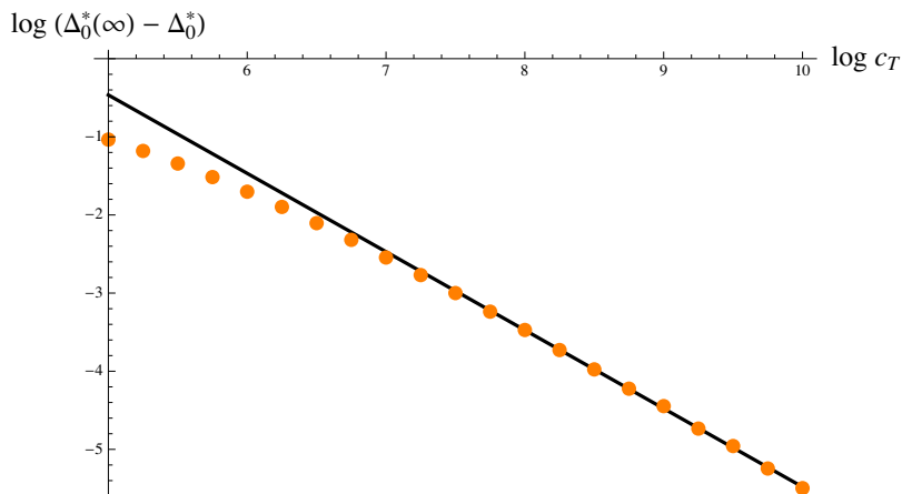
Figure 2. Upper bounds on \Delta_0^* (the smallest conformal dimension of a spin-0 long multiplet appearing in the \mathcal{O}_{35_c} \times \mathcal{O}_{35_c} OPE) for large values of c_T . The bounds are computed with j_{\max} = 20 and \Lambda = 19 . The long multiplets of spin j > 0 are only restricted by unitarity. The best fit for the last ten points (shown in black) is \log(\Delta_0^*(\infty) - \Delta_0^*) = 4.55 - 1.00 \log c_T .
