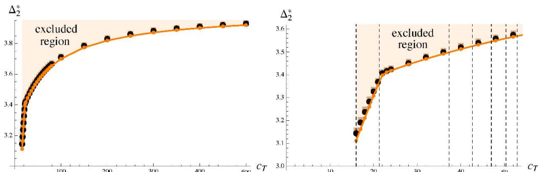
Figure 3. Upper bounds on \Delta_2^* , which is the smallest conformal dimension of a long multiplet of spin-2 appearing in the \mathcal{O}_{35_c} \times \mathcal{O}_{35_c} OPE. The long multiplets of spin j \neq 2 are only restricted by unitarity. These bounds are computed with j_{\max} = 20 and \Lambda = 19 (orange), \Lambda = 17 (black), and \Lambda = 15 (light brown). The plot on the right is a zoomed-in version of the plot on the left. The dashed vertical lines correspond to the values of c_T in table 9.
