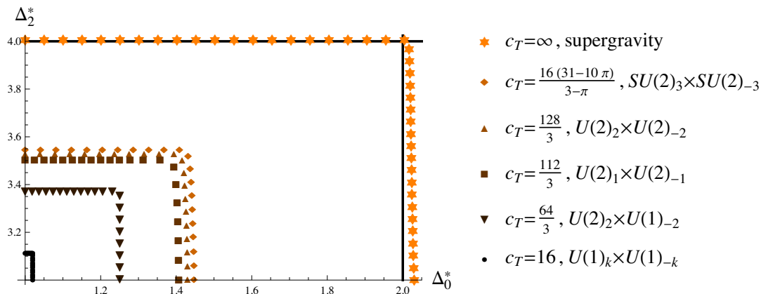
Figure 4. Combined upper bounds on \Delta_0^* and \Delta_2^* , which are the smallest scaling dimensions of spin-0 and spin-2 long multiplets appearing in the \mathcal{O}_{35_c} \times \mathcal{O}_{35_c} OPE. The long multiplets of spin j > 2 are only restricted by unitarity. The bounds are computed with j_{\max} = 20 and \Lambda = 19 . The solid lines correspond to the expected scaling dimensions in ABJM theory at large N .
