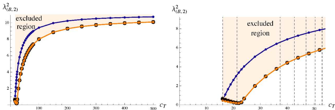
Figure 6. Upper bounds on \lambda_{(B,2)}^2 using only the unitarity assumption (in blue) or a more restrictive assumption on scaling dimensions of long multiplets of spin-0 in orange. (See main text.) These bounds are computed with j_{\max} = 20 and \Lambda = 19 . For the more restrictive bounds, we also show the corresponding values computed with \Lambda = 17 (in black) and \Lambda = 15 (in light brown). The plot on the right is a zoomed-in version of the plot on the left. The dashed vertical lines correspond to the values of c_T in table 9.
