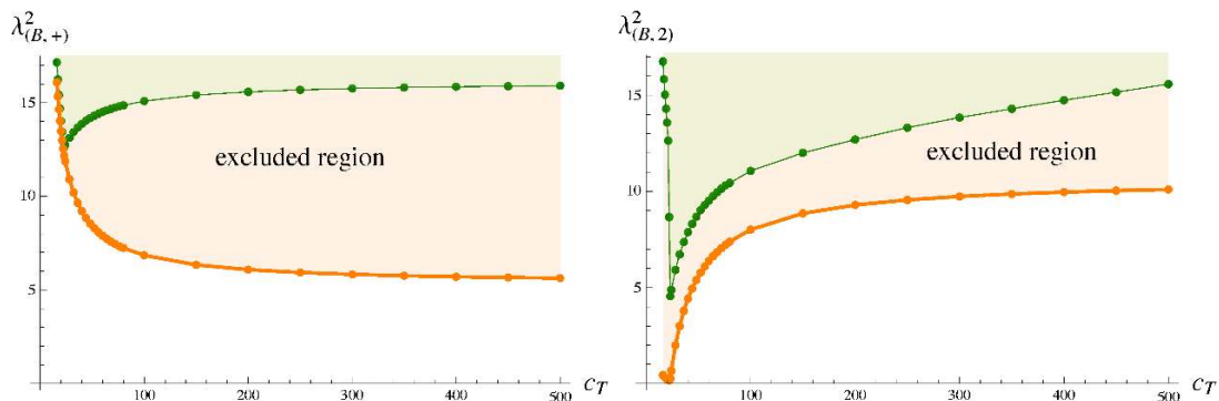
Figure 7. Upper bounds on \lambda_{(B,+)}^2 and \lambda_{(B,2)}^2 computed either using derivatives w.r.t. x and \bar{x} of d_2 (see (6.1)) and holomorphic derivatives of d_1 (in orange), or using only derivatives of d_2 (in green). These bounds are obtained with j_{\max} = 20 , \Lambda = 19 , and a more restrictive set of assumptions on \Delta_0^* only.
