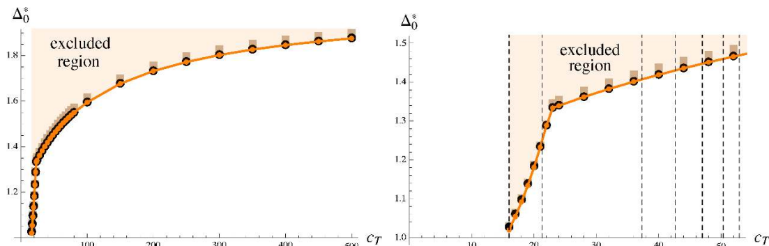
Figure 1. Upper bounds on \Delta_0^* , which is the smallest conformal dimension of a long multiplet of spin-0 appearing in the \mathcal{O}_{35_c} \times \mathcal{O}_{35_c} OPE. The long multiplets of spin j > 0 are only restricted by unitarity. These bounds are computed with j_{\max} = 20 and \Lambda = 19 (orange), \Lambda = 17 (black), and \Lambda = 15 (light brown). The plot on the right is a zoomed-in version of the plot on the left. The dashed vertical lines correspond to the values of c_T in table 9.
