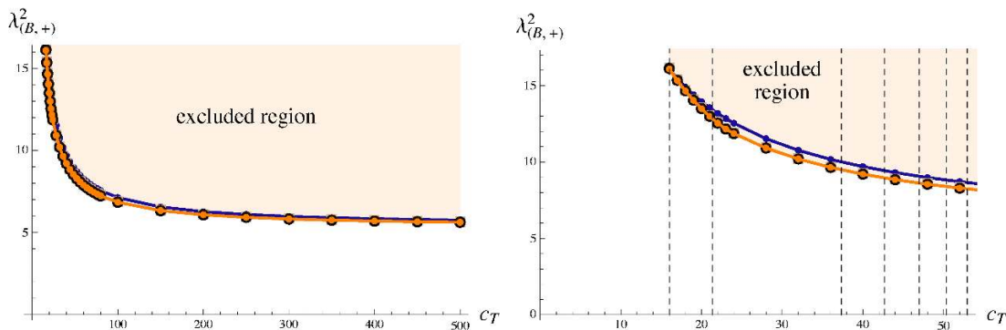
Figure 5. Upper bounds on \lambda_{(B,+)}^2 using only the unitarity assumption (in blue) or a more restrictive assumption on scaling dimensions of long multiplets of spin-0 in orange. (See main text.) These bounds are computed with j_{\max} = 20 and \Lambda = 19 . For the more restrictive bounds, we also show the corresponding values computed with \Lambda = 17 (in black) and \Lambda = 15 (in light brown). The plot on the right is a zoomed-in version of the plot on the left. The dashed vertical lines correspond to the values of c_T in table 9.
