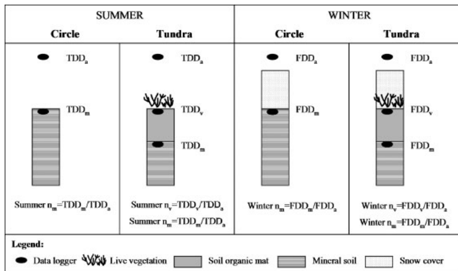
Figure 3 Diagram showing location of the temperature loggers in nonsorted circles and adjacent tundra. For each logger position, the derived thawing degree-day sums for air (TDD a ), under live vegetation (TDD v ) and at the top of the mineral soil (TDD m ) are indicated for summer, and freezing degree-day sums for air (FDD a ), under live vegetation (FDD v ) and at the top of the mineral soil (FDD m ) are indicated for winter. Calculations for the n-factor as an index of thermal insulation under live vegetation ( n_v ) and at the mineral soil surface ( n_m ) are shown.
