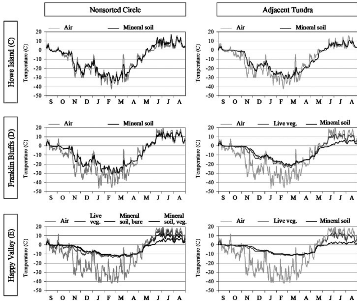
Figure 4 Daily mean temperatures from 1 September 2003 to 31 August 2004 for air (2 m height), under live vegetation and at the surface of the mineral soil for nonsorted circles and adjacent tundra at the three study sites.
