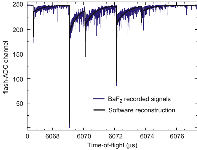
Fig. 3. Digitized buffer containing five \text{BaF}_2 signals that are identified and reconstructed by the PSA routine.
