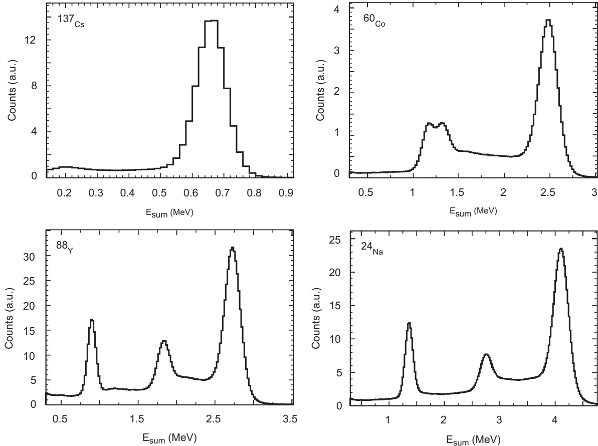
Fig. 4. TAC response to the standard \gamma -ray sources ^{137}\text{Cs} , ^{60}\text{Co} , ^{88}\text{Y} and ^{24}\text{Na} .
