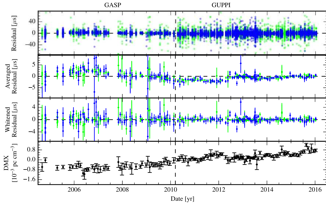
Figure 15. Timing summary for PSR J1012+5307. The colors are defined as follows. Blue: 1.4 GHz. Purple: 2.1 GHz. Green: 820 MHz. Orange: 430 MHz. Red: 327 MHz. In the top panel, individual points are semi-transparent; darker regions arise from the overlap of many points.
