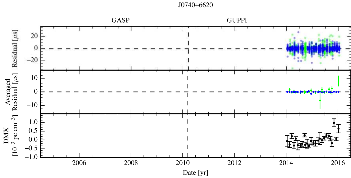
Figure 13. Timing summary for PSR J0740+6620. The colors are defined as follows. Blue: 1.4 GHz. Purple: 2.1 GHz. Green: 820 MHz. Orange: 430 MHz. Red: 327 MHz. In the top panel, individual points are semi-transparent; darker regions arise from the overlap of many points.
