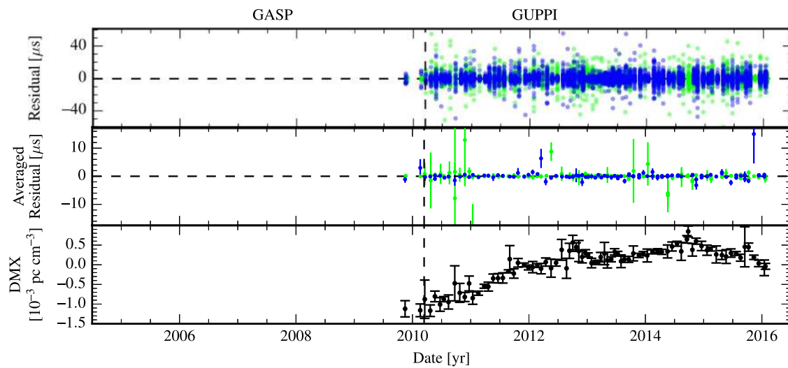
Figure 16. Timing summary for PSR J1024-0719. The colors are defined as follows. Blue: 1.4 GHz. Purple: 2.1 GHz. Green: 820 MHz. Orange: 430 MHz. Red: 327 MHz. In the top panel, individual points are semi-transparent; darker regions arise from the overlap of many points.
