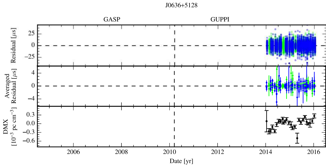
Figure 11. Timing summary for PSR J0636+5128. The colors are defined as follows. Blue: 1.4 GHz. Purple: 2.1 GHz. Green: 820 MHz. Orange: 430 MHz. Red: 327 MHz. In the top panel, individual points are semi-transparent; darker regions arise from the overlap of many points.
