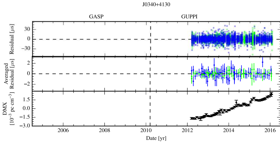
Figure 9. Timing summary for PSR J0340+4130. The colors are defined as follows. Blue: 1.4 GHz. Purple: 2.1 GHz. Green: 820 MHz. Orange: 430 MHz. Red: 327 MHz. In the top panel, individual points are semi-transparent; darker regions arise from the overlap of many points.
