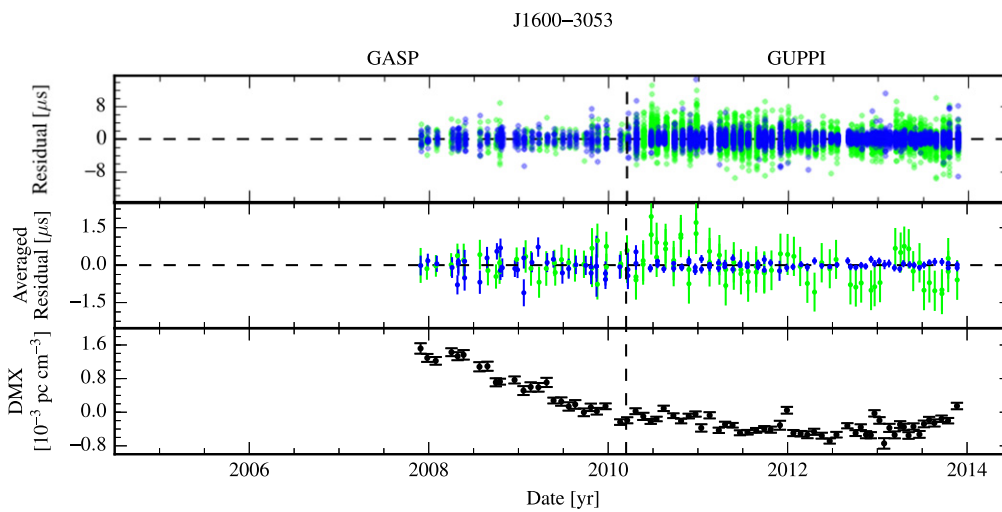
Figure 16. Timing summary for PSR J1600–3053. Colors are blue: 1.4 GHz, purple: 2.3 GHz, green: 820 MHz, orange: 430 MHz, red: 327 MHz. In the top panel, individual points are semi-transparent; darker regions arise from the overlap of many points.
