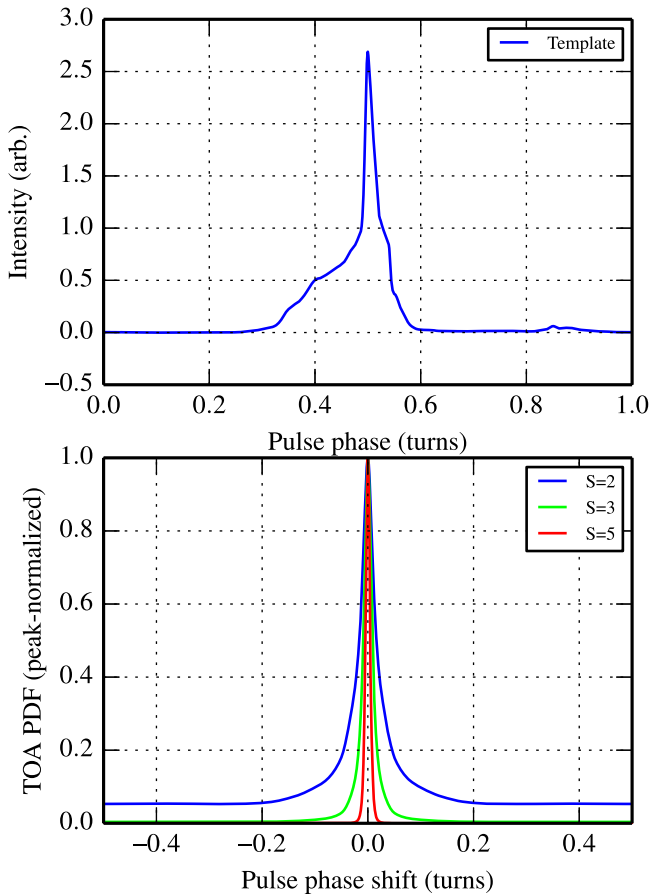
Figure 5. Upper panel: 1.4 GHz template profile for J1455–3330. Lower panel: expected pulse phase shift distributions for several values of S/N , from Equation (13). For plot clarity these are normalized to 1 at \phi = 0 , rather than to constant integrated area. This shows the evolution of the distribution from nearly Gaussian at higher S/N ( S = 5 ) to clearly non-Gaussian at low- S/N ( S = 2 ).
