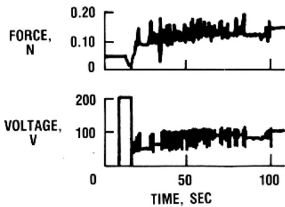
FIGURE 9. - ARCJET STARTING PHENOMENA. (35)
