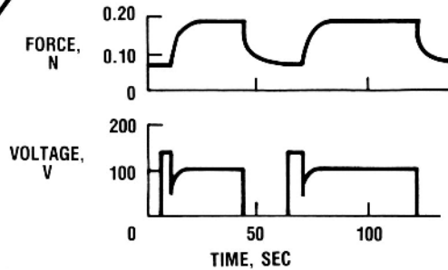
FIGURE 9. - ARCJET STARTING PHENOMENA. (35)
