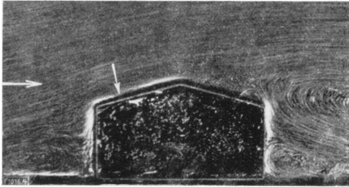
Fig. 2. Flow past model house with sloping roof.
