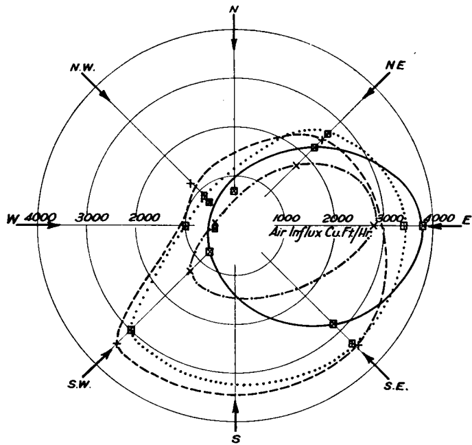
Text-fig. 7. Dependence of the rate of influx of air on the direction of wind. For speed groups 3\frac{1}{2} -6 m.p.h. and 6\frac{1}{2} -9 m.p.h. for 50 sq.in. flue and 50 sq.in. grating. Room B 1360 cu.ft. Wall containing grating and windows facing east.
