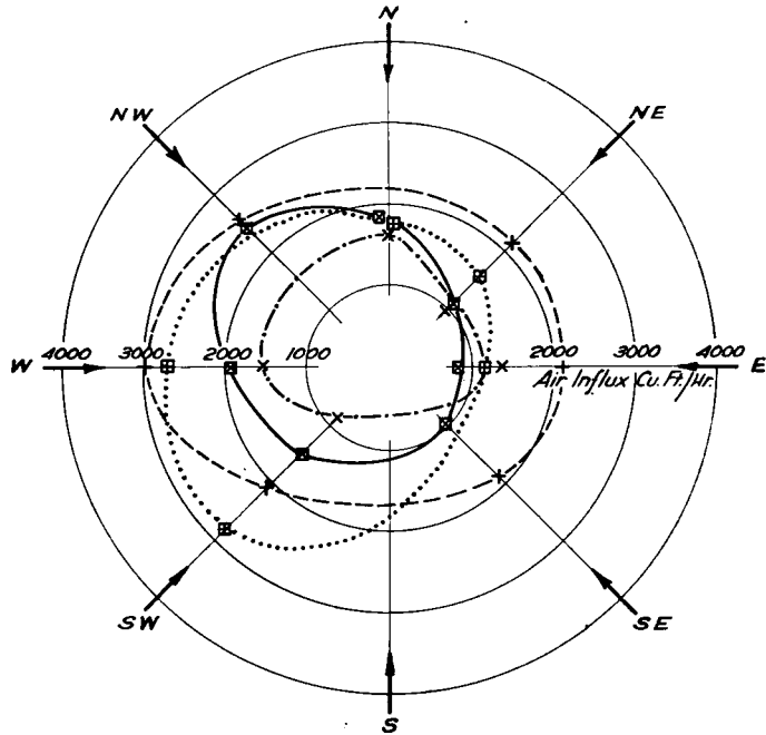
Text-fig. 6. Dependence of the rate of influx of air on the direction of wind. For speed groups 3\frac{1}{2} -6 m.p.h. and 6\frac{1}{2} -9 m.p.h. for 50 sq.in. flue and 50 sq.in. grating. Room A 1640 cu.ft. Wall containing grating and windows facing south-west.
