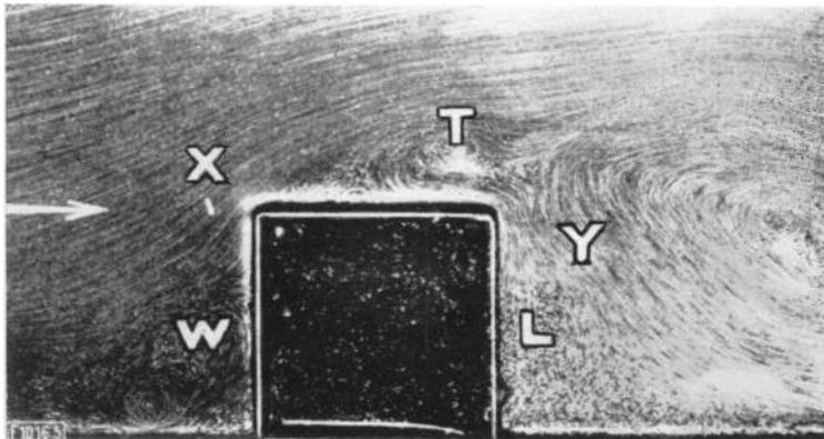
Fig. 3. Flow past model house with flat roof. Lettering on the photograph has been added by the author.
