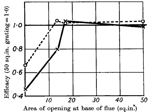
Text-fig. 5. Efficacy of flue openings, relative to 50 sq.in. grating. (Averages for all observed wind velocities. See Table 3 and derivation.)
