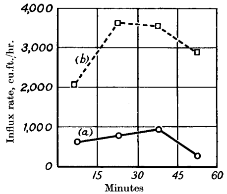
Text-fig. 3. Variation of influx rate during test period of one hour. Room A.
