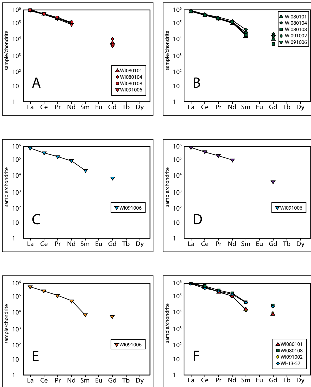
Fig. 26: A-F: Chondrite-normalized REE-profiles for the major REE-bearing minerals in the Wicheeda carbonatite. A. Bastnäsite-(Ce). B. Parisite-(Ce). C. Synchysite-(Ce). D. Ancylyte-(Ce) E. Cordylite-(Ce). F. Monazite-(Ce). The chondrite values were taken from McDonough and Sun (1995).
