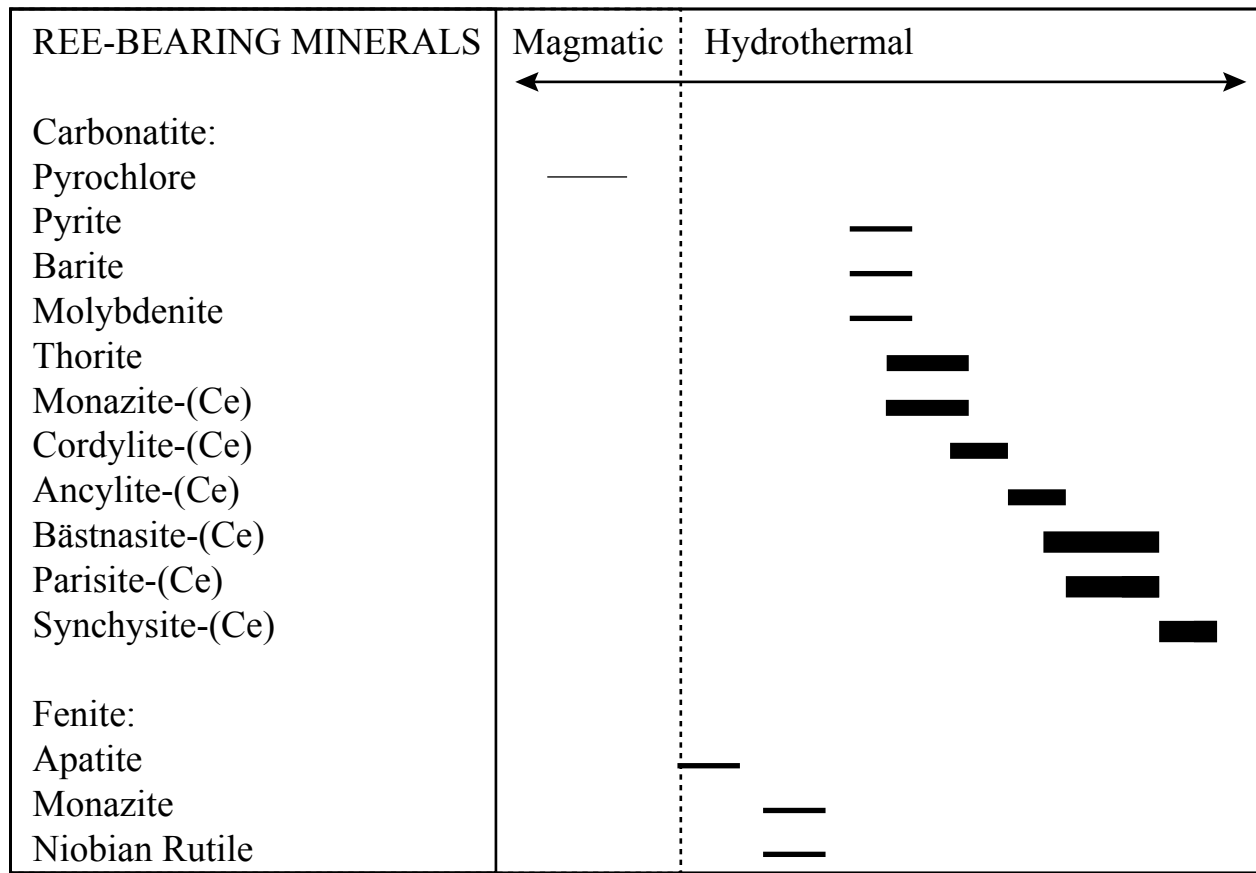
Fig. 10: Paragenetic diagram showing the order of crystallization of the main REE-bearing and associated minerals in the Wicheeda carbonatite. The line widths indicate the relative abundances of the minerals.
