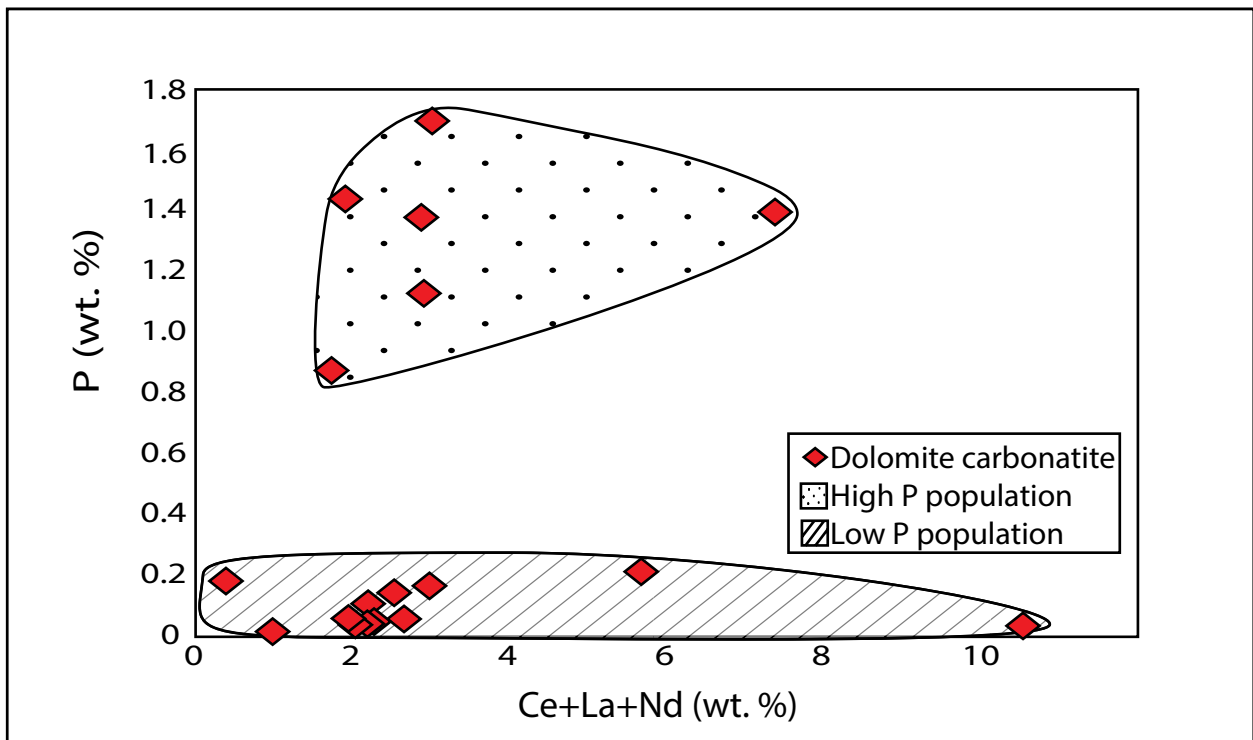
Fig. 19: A. The concentration of Ce+La+Nd (wt.%) as a function of F concentration (wt. %) in the dolomite carbonatite. The trend line illustrates the linear relationship between F and LREE contents. B. The concentration of Ce+La+Nd (wt.%) as a function of P concentration in the dolomite carbonatite. The data indicate the presence of a high P population (representing fluorapatite-bearing fenite xenoliths), and a low P population (xenolith-free).
