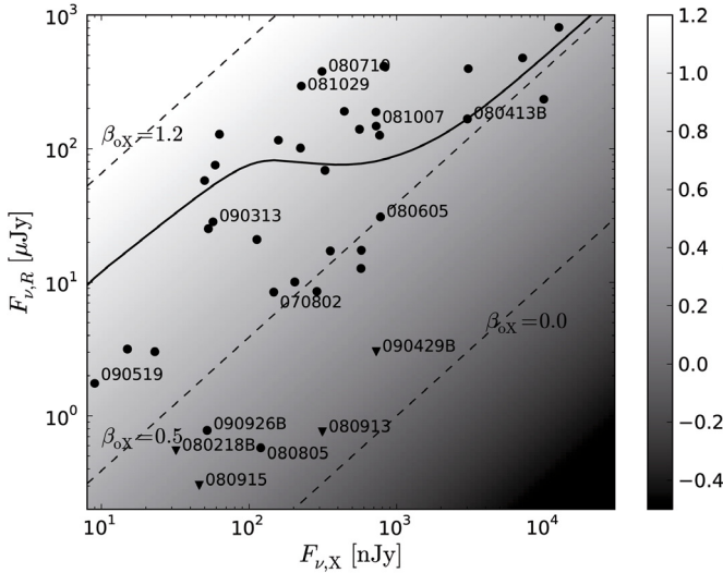
Fig. 2. The distribution of our sample GRBs in the plane of R -band flux over X-ray flux Jakobsson et al. (2004). For GRB 080413B we show as a thick solid line the temporal evolution of \beta_{\text{OX}} with time during the first 2 days of the afterglow evolution (from top to bottom left).
