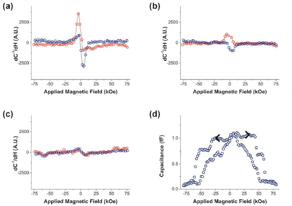
Figure 4: Probing the existence and relative magnitude of P^2M^2 coupling in PZTFT. Plots of dC^{-1}/dH as a function of magnetic field applied along the [001]_{pc} , [110]_{pc} and [\bar{1}10]_{pc} directions (a, b and c respectively) in the single crystal lamella coplanar capacitor, at 150K. Red data points are for increasing field and blue data points for decreasing field. For magnetic fields applied along [001]_{pc} (parallel to the electrode-dielectric interface and in the plane of the lamella), the plot is similar to that of -M(dM/dH) in figure 3(c). This is consistent with measurable P^2M^2 coupling. The magnitude of the P^2M^2 coupled response is reduced, but still evident, when magnetic fields are along [110]_{pc} (in the plane of the lamella and perpendicular to the electrode-dielectric interface) in (b) and almost imperceptible when the field is along [\bar{1}10]_{pc} (perpendicular to the plane of the lamella) in (c). The minor influence of symmetric P^2M^2 behaviour for fields along [\bar{1}10]_{pc} is consistent with the observed magnetic field-induced ferroelectric switching, which requires asymmetric coupling terms (such as PM ). Capacitance still shows a significant dependence on magnetic field in this orientation (not explained by PM coupling), even at room
