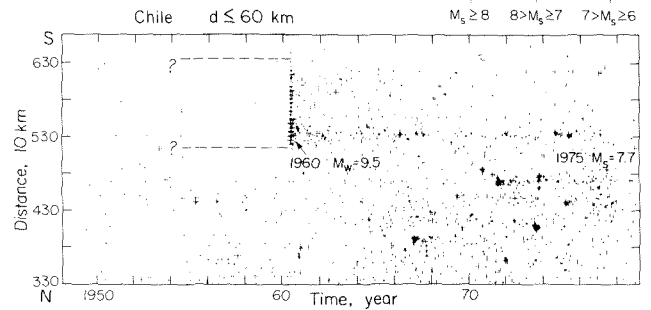
Fig. 7. Space-time plot of seismicity for Chile. See caption for Fig. 3 for details.
