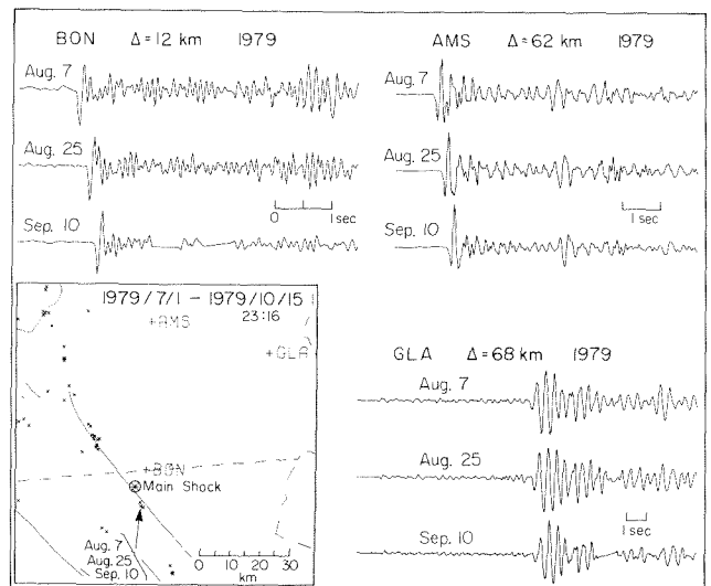
Fig. 19. Wave forms of three foreshocks of the 1979 Imperial Valley earthquake recorded at three stations.
