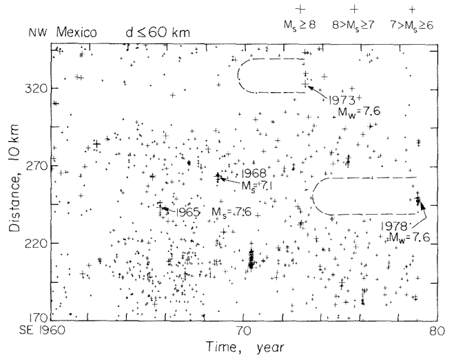
Fig. 3. Space-time plot of seismicity for Mexico obtained from the NOAA catalog (See Fig. 2 for the location). Dotted curves encircle the period of quiescence. The magnitude ranges for the larger symbols are indicated in the figures. The magnitude ranges for the events smaller than 6 are not indicated but the size of the symbols is approximately proportional to the magnitude.
