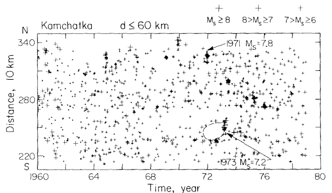
Fig. 13. Space-time plot of seismicity for the Kamchatka region for the period 1960 to 1978. For details, see caption for Fig. 3.
