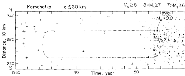
Fig. 12. Space-time plot of seismicity for the rupture zone of the 1952 Kamchatka earthquake. For details, see caption for Fig. 3.
