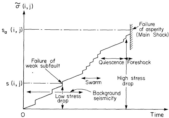
Fig. 18. Temporal variation of stress \tilde{\sigma} at a subfault. A step-wise increase is caused by failure of another weaker subfault.
