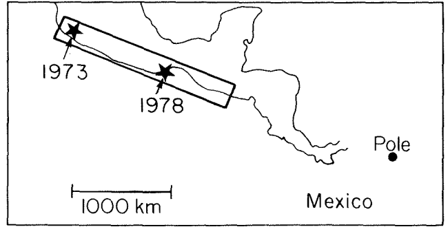
Fig. 2. Index map for Mexico. All the events shallower than 60 km which occurred in the box are shown in Fig. 3. The asterisks show the location of the 1973 Colima earthquake and the 1978 Oaxaca earthquake. The location of the pole is arbitrary, and the scale refers to the middle of the figure.
