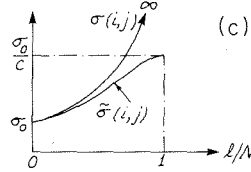
Fig. 15. Schematic figure showing a unit fault containing an asperity (a), the distribution of strength of subfaults within the asperity and the surrounding area (b), and the stress \tilde{\sigma} on subfaults (c).
