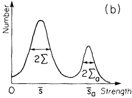
Fig. 15. Schematic figure showing a unit fault containing an asperity (a), the distribution of strength of subfaults within the asperity and the surrounding area (b), and the stress \tilde{\sigma} on subfaults (c).
