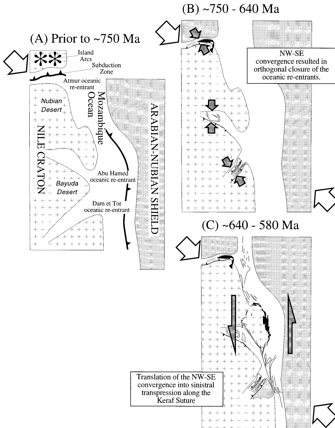
Figure 7. A three-step, map-like model illustrating the tectonic evolution of the pre-Kerf and Kerf structures as products of oblique collision between the Arabian-Nubian Shield and the Nile Craton. (a) Pre-collision configuration of the Arabian-Nubian Shield and the Nile Craton with part of the Mozambique Ocean between them. Note the presence of oceanic reentrants along the present extent of the Atmur-Delgo Suture and the Abu Hamed and Dam et Tor Fold/Thrust Belts. The Atmur-Delgo reentrant is different from the Abu Hamed and Dam et Tor reentrants in that it is associated with a N-dipping subduction zone. (b) Closure of the oceanic reentrants due to oblique convergence. (c) Closure of the oceanic basin between the Arabian-Nubian Shield and the Nile Craton. The NW-SE convergence was translated into sinistral transpression along the Kerf Suture.
