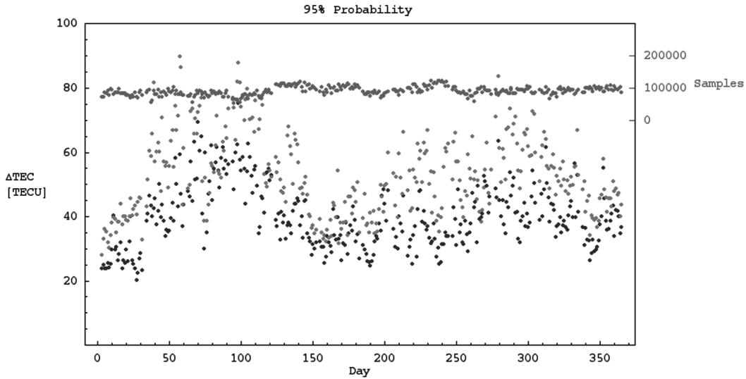
Fig. 3. 95 percentile (95% probability) of the cumulative distribution for global daily mis-modelling (difference between an experimental and its corresponding modelled slant TEC) for the ICA model (gray) and NeQuick 2 model (black). In the top part of the figure the corresponding samples used in each daily calculation is given.
