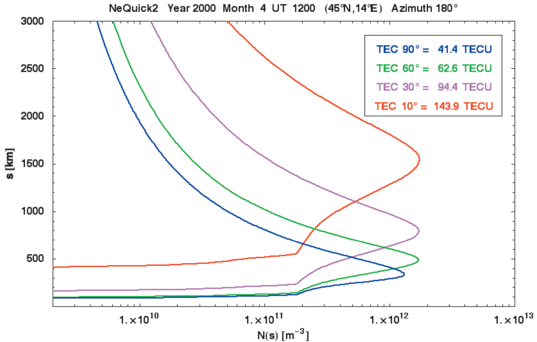
Fig. 2. Example of NeQuick 2 profiles and TEC along ray-paths. Different colors correspond to different path elevation angles. 90^\circ means vertical profile and TEC.
