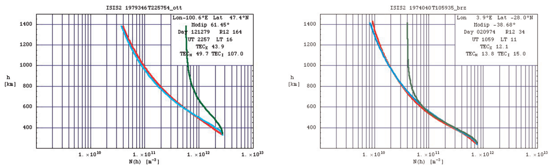
Fig. 1. Examples of comparisons among electron density topside profiles. Red curves correspond to ISIS 2 experimentally derived profiles. Green corresponds to IRI-2000 profiles and light-blue are NeQuick 2 profiles.
