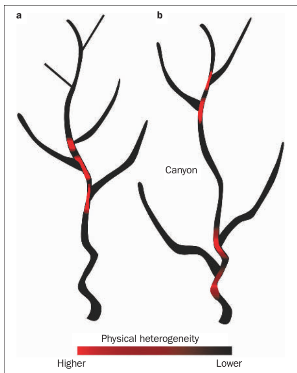
Figure 6. Local network geometry (kilometer scale) varies in response to the size, spacing, and confluence angles of intersecting tributaries, which reflect underlying geologic structure, topography, and erosion history. Different local geometries are expected to lead to different patterns of physical heterogeneity, linked to tributary confluences. (a) With a number of large tributaries near the center of the network, confluence-related heterogeneity is concentrated in a central, sediment-producing region. This pattern is characteristic of watersheds located along mountain fronts and abutting depositional plains. (b) When major tributaries are separated by canyons, the associated areas of physical heterogeneity are divided as well.
