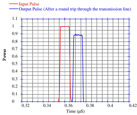
Figure 2. Performance of the transmission line that connects the pulse compressor to the accelerator.
