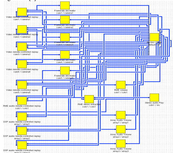
Figure 2- Executable Smart Data Flow System graph for Meeting Room data processing and review.
