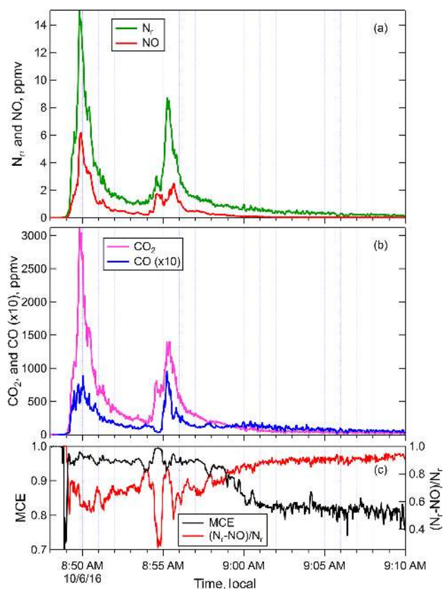
Figure 2. Timelines of the (a) N_r and NO, (b) \Delta\text{CO}_2 and \Delta\text{CO} , and (c) MCE and (N_r - \text{NO}) / N_r measured during Fire 004, a ponderosa pine realistic mix sample. Note that \Delta\text{CO} is plotted at \times 10 the measured abundance for clarity.
