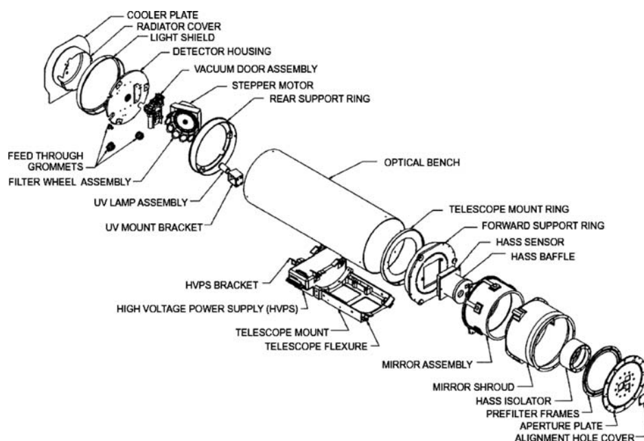
Figure 2. Instrument exploded view (GOES I-M Data Book (1996)).
