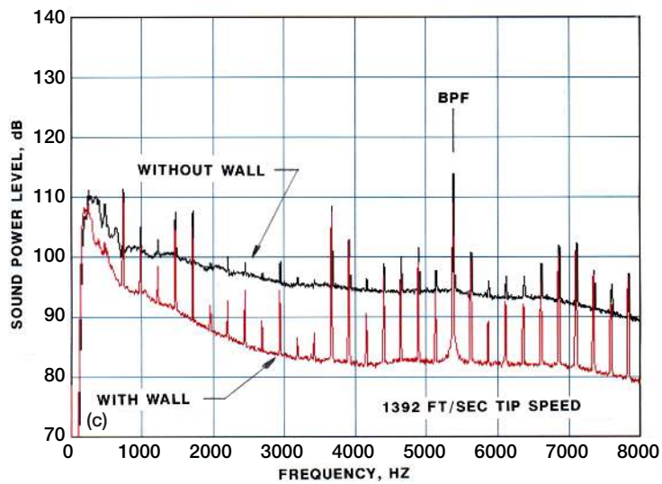
Figure 17.—Sound power level for 83 degrees and forward. Quiet high-speed fan (a) without wall, (b) with wall, and (c) composite.
