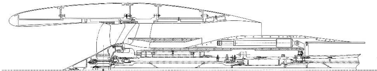
Figure 1.—Baseline fan. (a) Photograph. (b) Cross section.
