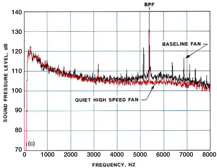
Figure 10.—Spectra at 136.4 degrees, 1392 ft/sec tip speed. (a) Baseline fan. (b) Quiet high-speed fan. (c) Composite.
