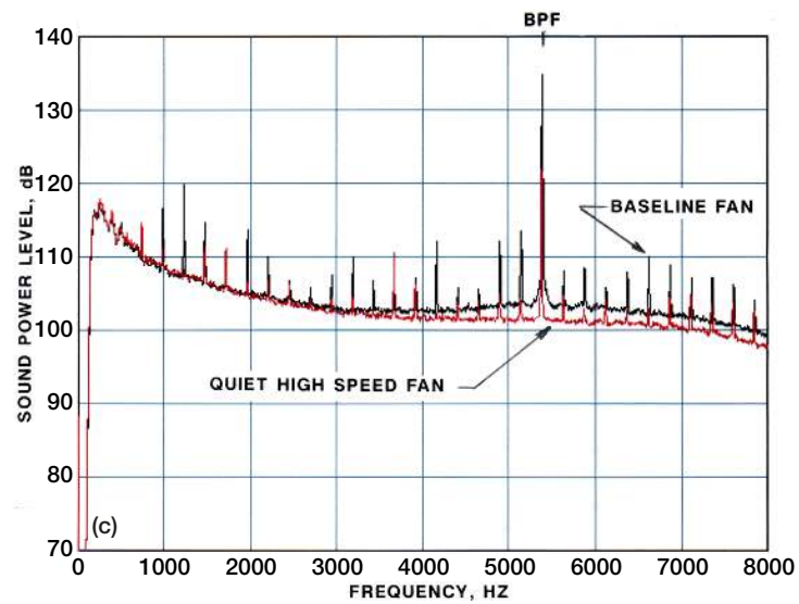
Figure 12.—Total sound power level at 1392 ft/sec tip speed. (a) Baseline fan. (b) Quiet high-speed fan. (c) Composite.
