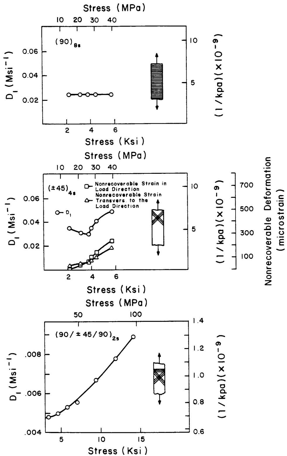
Fig. 7.11 Comparison of the Power Law Coefficient D_1 Obtained for Three Different Laminates at 320°F (160°C)
