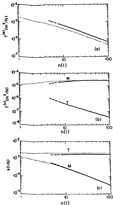
Fig. 1a-c. a Elastic transfer function T^{(e)} , b viscous transfer function T^{(v)} and c inverse relaxation time s as function of angular order n according to compressible solution (solid) or incompressible approximation (dotted); symbols M and T denote relaxation mode
