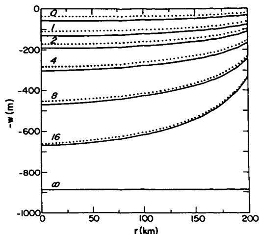
Fig. 2. Vertical surface displacement w as function of distance r from load axis for several times (in units of ka ) after emplacement of load according to compressible solution (solid) and incompressible approximation (dotted)
