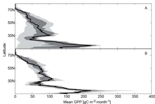
Fig. 5. North American multi-year mean (2000–2005) GPP from (A) the NACP regional and continental interim synthesis (RCIS) and (B) the MsTMIP simulations for 5 models (CLM, DLEM, LPJ, ORCHIDEE-LSCE, and VEGAS). On each panel, the solid line shows the median of the multi-model ensemble, the darker shaded area shows the interquartile range; and the lighter band shows the full range in estimates.
