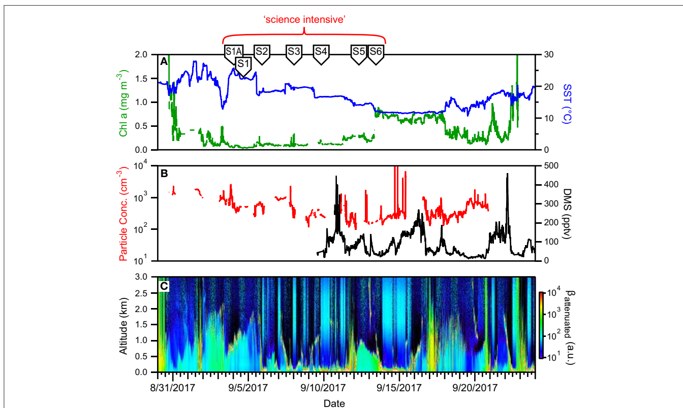
FIGURE 12 | Ocean and atmosphere properties as a function of campaign date during NAAMES 3. (A) Surface chlorophyll concentration (green line) and sea surface temperature (SST; blue line) as a function of hours along ship transit. (B) Particle number concentration (red line) and dimethylsulfide gas mixing ratio (black line) along the ship transit. (C) Attenuated backscatter curtain in arbitrary units as detected by the ship-based ceilometer along the ship transit. The record begins on 8/30/2017 at 41° 9' N, 70° 54' W on the outbound transit and ends on 9/24/2017 at 41° 25' N, 66° 59' W on the return transit. Red bracket = “science intensive” segment of transit. Labeled symbols at top of panel indicate ship location at the beginning of each primary station (S1A–S6).
