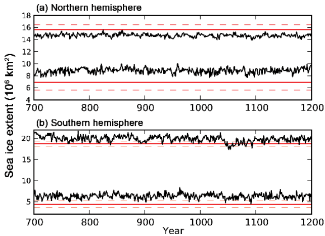
Fig. 4. Time series of (a) northern and (b) southern hemispheric sea ice extent ( 10^6 \text{ km}^2 ) for March and September in piControl. Black lines show simulated annual mean time series and red lines show observed annual mean and \pm 2 sd for the years 1979–2005 (data from NSIDC, Fetterer et al., 2009).
