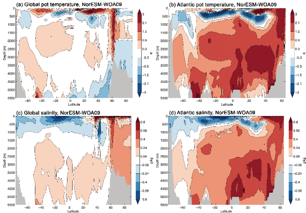
Fig. 14. Difference between NorESM HistoricalI 1976–2005 and WOA9 zonal mean potential temperature (a, b) and salinity (c, d). Left and right panels are for global and Atlantic domains, respectively.
