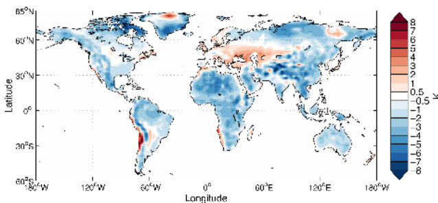
Fig. 6. Comparison of simulated air temperature at reference height over the ground surface with NorESM for 1976–2005 (Historical1) with the CRU TS3.1 (Mitchell and Jones, 2005) observational data set for the same period interpolated to the same grid using conservative remapping. Global bias error is -1.0868 K with a RMSE of 2.347 K.
