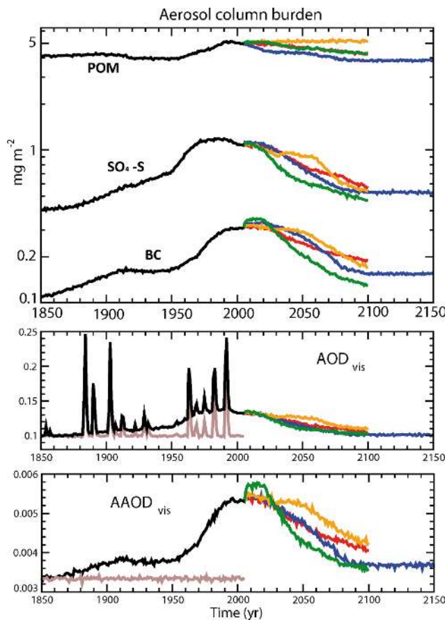
Fig. 2. Globally and annually averaged aerosol column burdens for particulate organic matter (POM), particulate sulphate as S ( \text{SO}_4\text{-S} ), and black carbon (BC) (upper panel), aerosol optical depth (AOD) (middle panel), and aerosol optical depth for absorption (AAOD) (lower panel) from 1850 onwards, calculated online in NorESM1-M. Curves for Historic1 from 1850 to 2005 are black. For scenario projections, green are RCP2.6 for 2005–2100, blue are RCP4.5 for 2005–2300 (negligible variations after 2150), orange are RCP6.0 for 2005–2100, and red are RCP8.5 for 2005–2100. The brown curves are contributions to AOD and AAOD in Historic1 by natural aerosols only, including prescribed stratospheric sulphate from explosive volcanoes.
