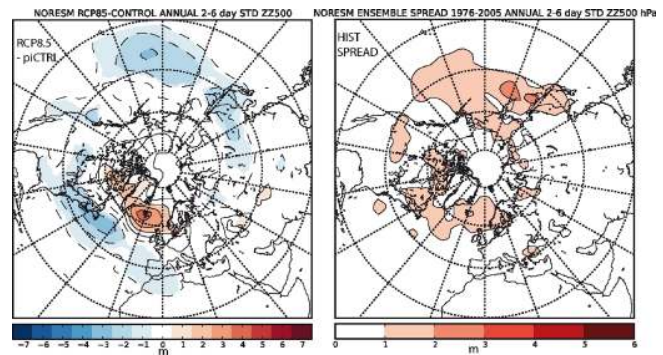
Fig. 12. NorESM1-M simulated change from 1976–2002 to 2071–2100 in NH extra-tropical storminess, diagnosed as described in Fig. 11, using the RCP8.5 projection scenario (left). Colours indicate significant changes on the 95% confidence level. The right panel shows the standard deviation in the storminess amongst the three ensemble-members Historic1–3 for 1976–2005, revealing that the significant changes diagnosed in the left panel are considerably larger for the main maxima.
