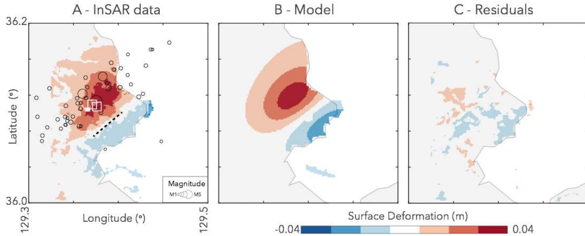
Fig. 3. DInSAR data and model: (A) Surface deformation (satellite Line-of-Sight displacements) obtained using DInSAR. seismicity and extrapolated fault trace are indicated by black circles and dashed line respectively. (B) Modeled surface deformation using a rectangular fault plane with the following parameters: Lat= 36.100; Lon=129.383 (center of the rectangular fault); Depth=4.3 km (upper edge of the fault) Strike (from North) = 225°; Dip (from horizon) = 75°; Length=~5 km; Width= ~1.6 km; Slip= ~1m; Rake=123°. (C) Difference between DInSAR data and model, i.e. Residuals. Standard deviation <0.5 cm, thus below the accuracy threshold of the measurements.
