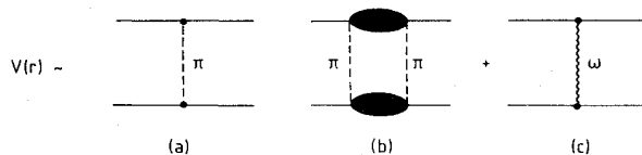
FIG. 1. Illustration of the nucleon-nucleon meson exchange potentials of shorter and shorter ranges. The two-pion exchange potential (b) involves nucleon excitations, crossed box diagrams, and \pi\pi interaction. It contains the scalar \sigma or \epsilon exchange as well as the \rho -meson exchange of the one-boson exchange potentials (OBEP).
