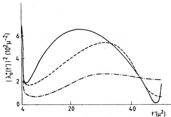
FIG. 13. Comparison of the NN\bar{\rightarrow}\pi\pi S -wave amplitude spectral function |\lambda_0^+(t)|^2 , where \lambda_0^+(t) = 4\pi/(M^2 - t/4)f_+^0(t) and where f_+^0 is the NN\bar{\rightarrow}\pi\pi S -wave helicity amplitude, the argument of which equals the S -wave \pi\pi phase shift for t \leq 16\mu^2 . Solid curve, Nielsen and Oades (1972) analysis; dot-dashed curve, Brown and Durso (1971) soft-pion constrained calculation; dashed curve, model used in Jackson, Riska, and VerWest's (1975) calculation, from which the figure is taken.
