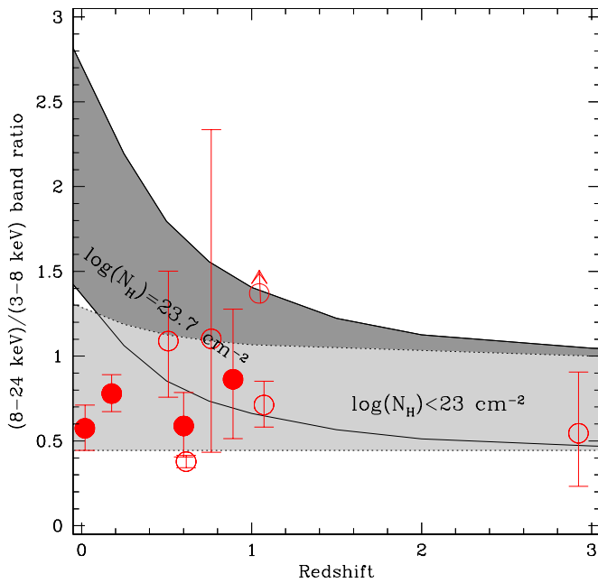
Figure 7. X-ray band ratio vs. redshift for the NuSTAR sources; see Figure 6 for a description of the symbols. The error bars indicate the 1\sigma uncertainty on the band ratio, which is calculated following the “numerical method” in Section 1.7.3 of Lyons (1991). The shaded regions show the range of expected band ratios for AGNs with N_{\text{H}} < 10^{23} \text{ cm}^{-2} and N_{\text{H}} \approx 5 \times 10^{23} \text{ cm}^{-2} , for an intrinsic spectral slope of \Gamma = 1.8 \pm 0.5 ; the dotted and solid curves indicate the maximum extents in band ratio for N_{\text{H}} < 10^{23} \text{ cm}^{-2} and N_{\text{H}} = 5 \times 10^{23} \text{ cm}^{-2} , respectively. The predicted band ratios were calculated using the RMF and ARF for NuSTAR J183443+3237.8 (see Section 2.1.5).
