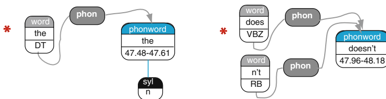
Fig. 1 Representation of the MS-State and Treebank3 Switchboard transcripts in NXT. Words in the Treebank3 transcript are represented by 'word' elements in one NXT layer, while those in the MS-State transcript are represented by 'phonword' elements in an independent layer. Representations of the same word in the two transcripts are linked by an NXT pointer labeled 'phon'. In some cases, such as contractions, words are tokenized differently in the two transcripts, so there may be multiple 'words' pointing at a 'phonword' or vice versa. Note that the star (*) shows that this structure is the expansion of the abbreviated word/phonword structure shown in Fig. 4
