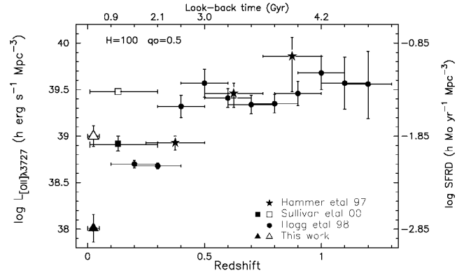
FIG. 2.—Evolution of the [O II] \lambda 3727 luminosity density of the universe. Both the observed and extinction-corrected values for the UCM sample are represented as filled and open triangles. Filled circles correspond to Hogg et al. (1998), filled stars are for the Hammer et al. (1997) values, and the filled and open squares are for the observed and extinction-corrected Sullivan et al. (2000) values.
