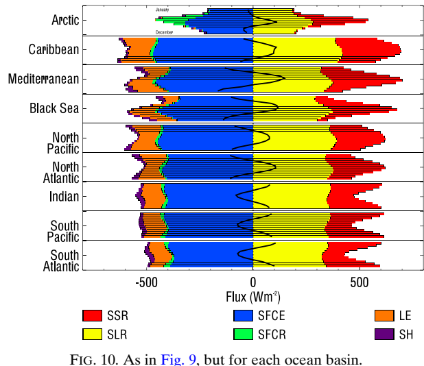
FIG. 10. As in Fig. 9, but for each ocean basin.
