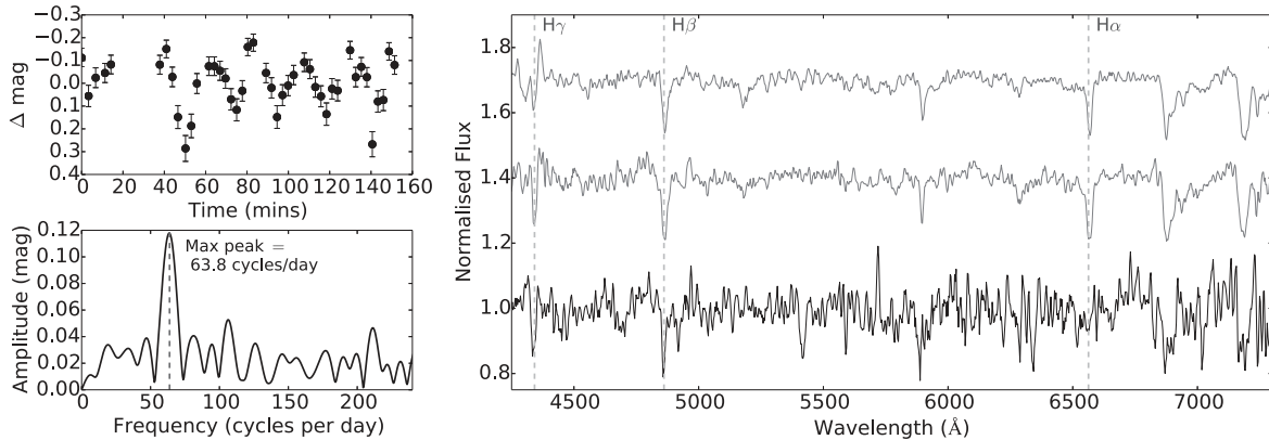
Figure 10. Properties of blue variable OW J074106.1–294811.0, including the OmegaWhite light curve (upper-left panel), the DFT power spectrum (lower-left panel), and the SALT-observed spectrum (right-hand panel). We plot the continuum-normalized spectra of the target (lower-black spectrum) and the spectra of two neighbouring stars for comparison (two upper grey spectra). All spectra have been smoothed by a running average of 3 and an offset has been applied for visualization purposes.
