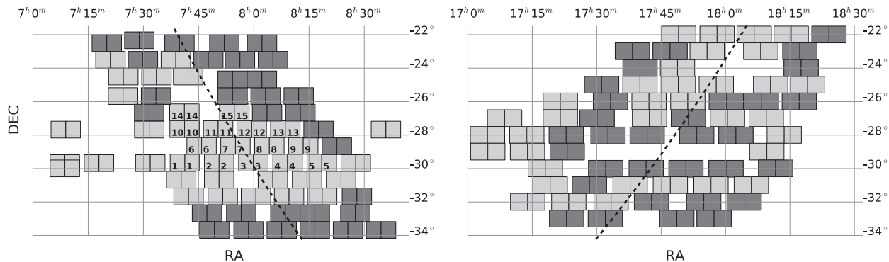
Figure 1. The two regions of OmegaWhite field pointings along the Galactic plane (dashed line), including the Galactic bulge region (right-hand panel). Fields are either observed (light grey, both panels), scheduled for semester 95 (dark grey, right-hand panel), or scheduled for semester 96 (dark grey, left-hand panel). Semester 88 field pairs are indicated by their identification number, and their respective co-ordinates are listed in Table A1.
