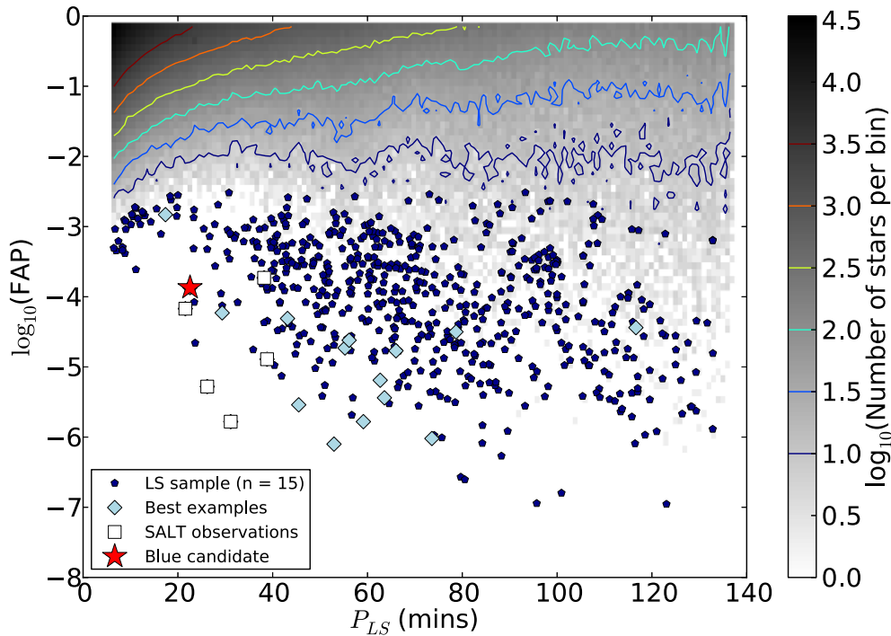
(b) Variable stars in ESO semester 88.
