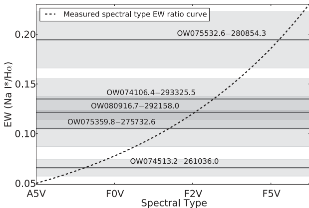
Figure 9. EW ratios of Na I doublet (5896 Å, 5890 Å) to H \alpha for a range of spectral types. Measured EW ratios increase exponentially towards later spectral types (as shown by the dashed curved line). The measured EW ratio for each of the five SALT variables are shown by a line spanning all spectral types, with respective measurement uncertainties indicated by shading. Likely spectral classes for each SALT variable are listed in Table 7.
