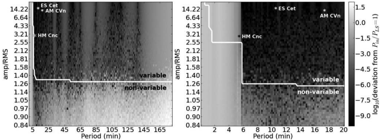
Figure 2. The logarithmic absolute deviation from P_{\text{in}}/P_{LS} = 1 , in period ( P_{\text{in}} ) and amp/rms space, sampled in one minute period bins (left-hand panel), and in 0.2 min period bins (right-hand panel). The region above and to the right of the white solid line indicates where sources have \log_{10}(\text{FAP}) < -2.5 , and are therefore considered variable at the 3\sigma level. The location of three short period (HM Cnc, ES Cet, and AM CVn) are each indicated by a star in both panels.
