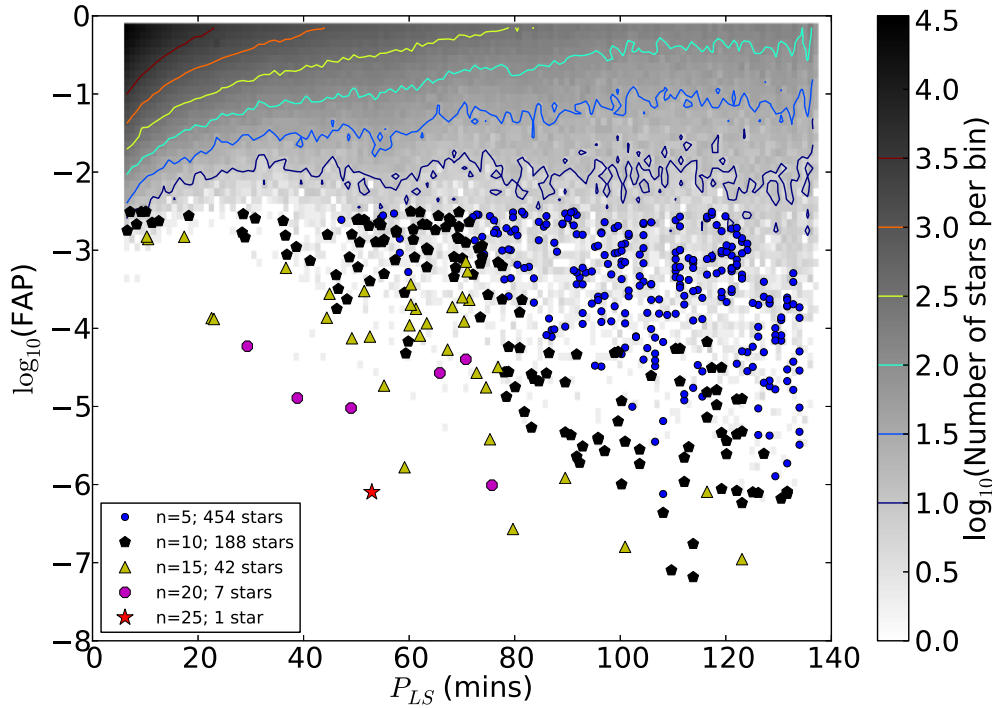
(a) Variable stars in Field OW_88D.1a.
