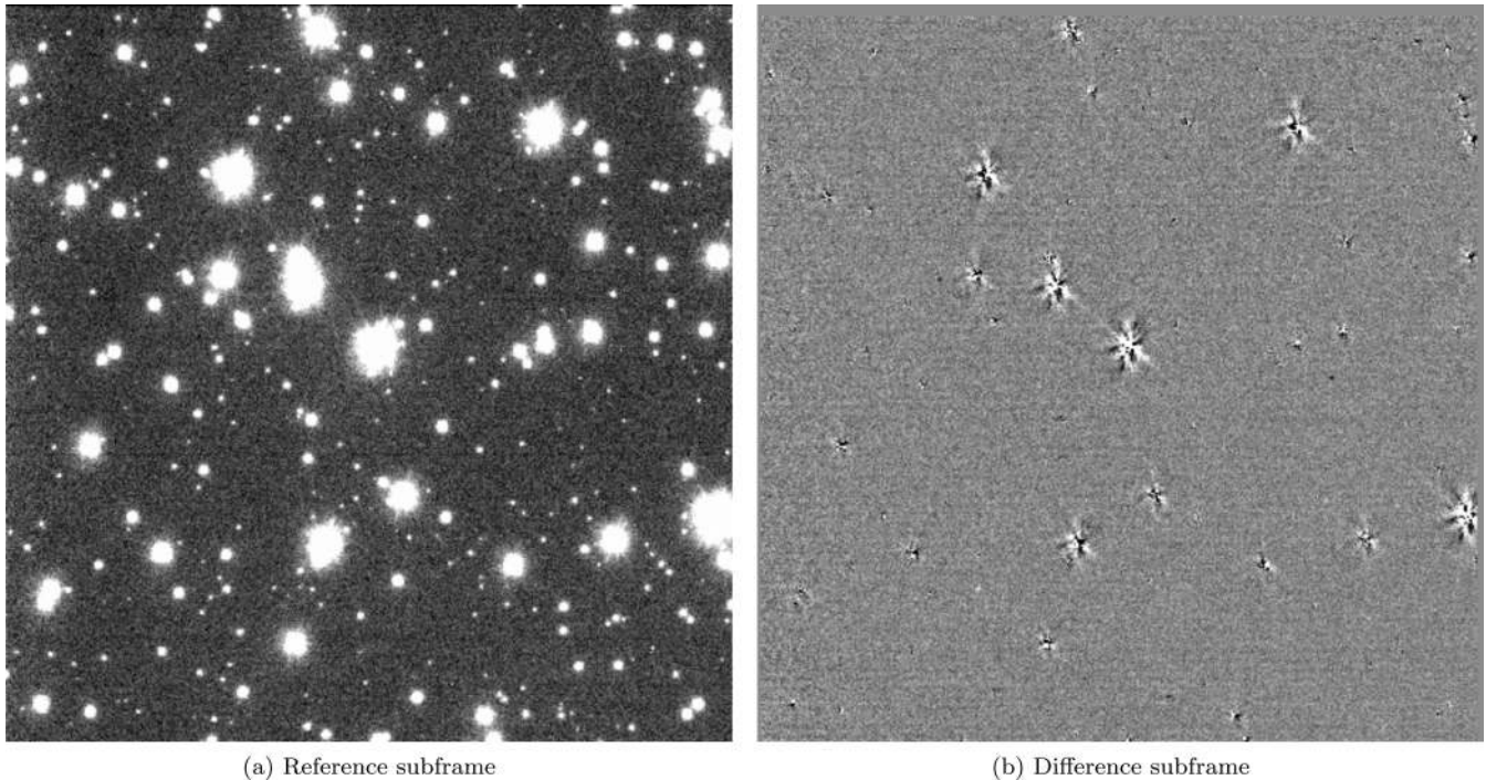
Figure 3. Difference subframe (right-hand panel) obtained after the reference subframe (left-hand panel) is convolved and then subtracted from an individual science subframe. Each subframe is 3.75 \text{ arcmin} \times 3.75 \text{ arcmin} . The residuals visible on the difference frame were caused by saturated stars.
