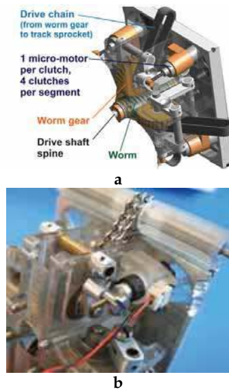
Fig. 26. Gear box and micro-clutches. a - CAD drawing, b - photograph In practice we implemented the micro-clutches as shown in Fig. 26. To disengage a track, a micro motor moves one link of a four-bar mechanism so that the worm gear is lifted off the worm. Micro-switches (not shown here) stop the micro-motor in two stable, self-locking positions. These positions correspond to the worm gear being fully engaged or disengaged from the worm.
