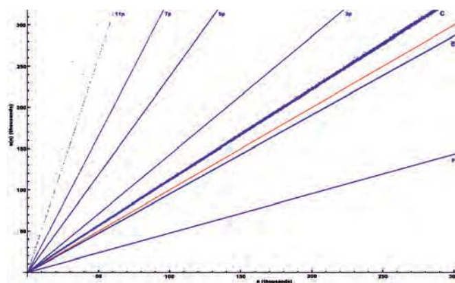
Figure 12. Scatterplot of the first 300,000 terms of the Yellowstone sequence. The primes lie on the lowest line (labeled “p”), the even numbers on the second line (“E”), the majority of the odd composite numbers on the third line (“C”), and the 3p , 5p , 7p , 11p, \dots points on the higher lines. The lines are not actually straight, except for the red line f(x) = x , which is included for reference.
