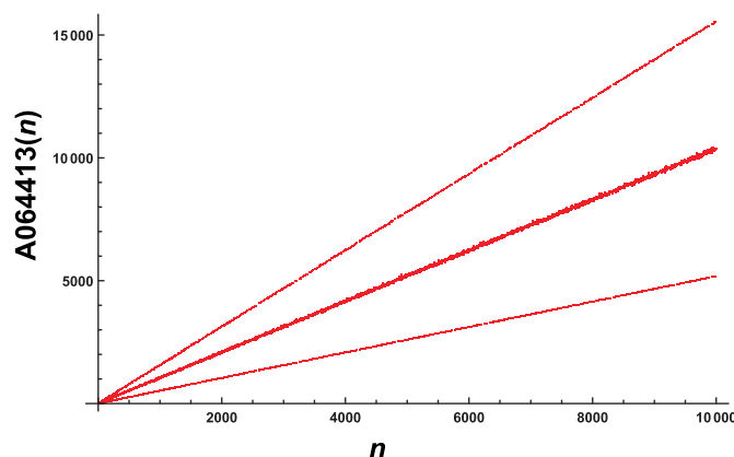
Figure 10. The first 10000 terms of the EKG sequence, so named because locally this graph resembles an EKG. Every number appears exactly once.
