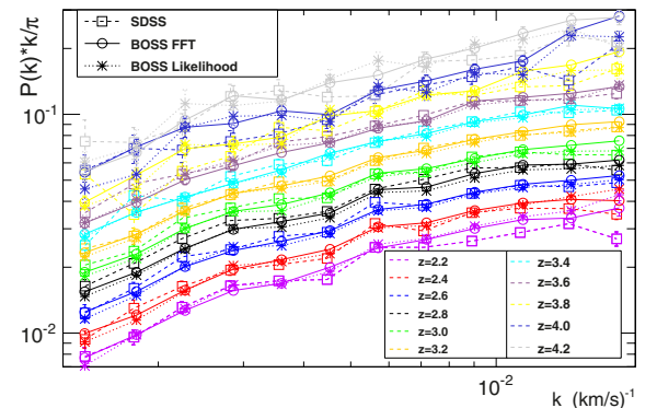
Fig. 21. Comparison of the 1D Ly \alpha forest power spectrum obtained in BOSS and in SDSS (see McDonald et al. 2006) over the redshift range, z = [2.1-4.3] . For BOSS, we show the results for the two methods, Fourier transform and likelihood, and we use the same k bins as in McDonald et al. (2006).
