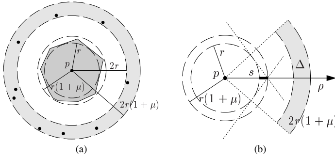
Fig. 3. (a) If the Voronoi cell C_p is (1 + \mu) -spherical with center p , then the neighboring sites must be in a spherical shell around p . (b) The sites of N(p) are densely spread in this spherical shell, since there must be a site inside the intersection \Delta between the spherical shell and any cone of angular radius 4\sqrt{\mu} .
