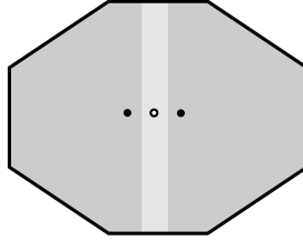
Fig. 2. Two points of Black can take over almost a complete cell of White.
