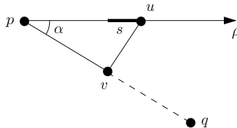
Fig. 4. Illustration of the proof of Lemma 8.
