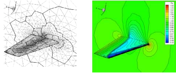
Fig. 11. elsA simulation of the M6 wing configuration: unstructured grid and static pressure iso-contours (Onera result from [15]).
