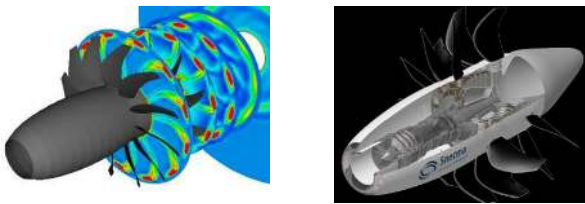
Counter rotating open rotor with 12 + 10 blades
