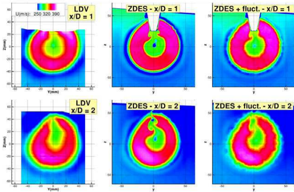
Fig. 10. Averaged velocity fields at x/D = 1 and 2. Left: LDV measurements – Middle: ZDES without RFG – Right: ZDES with RFG (Onera [34]).
