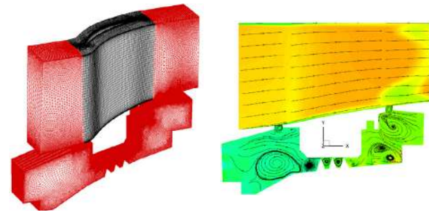
Fig. 12. elsA simulation in a shrouded stator : hybrid grid (unstructured blocks in red) and flowfield (streamlines in the cavity) (Onera result from [14]).
