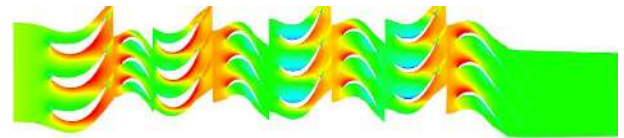
(a) Iso-absolute Mach number at mid-span
