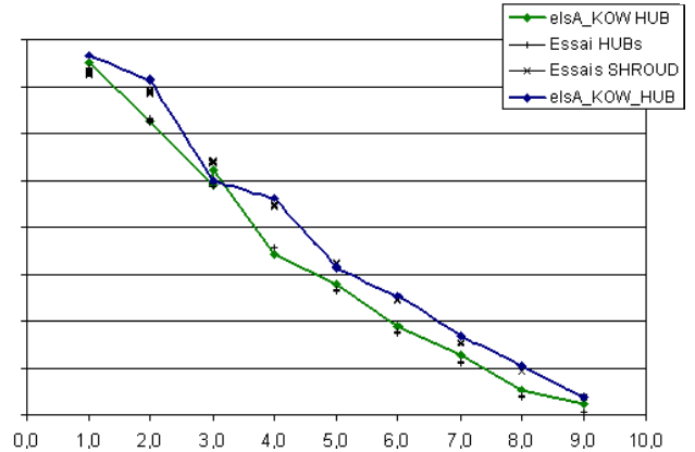
(b) Wall static pressure ( \Delta p = 2000 Pa) on the hub and on the shroud : comparison with experiment
